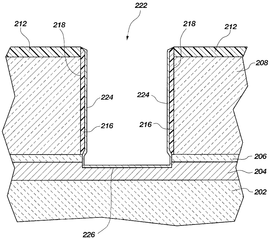
Fig. 14 (PRIOR ART)
