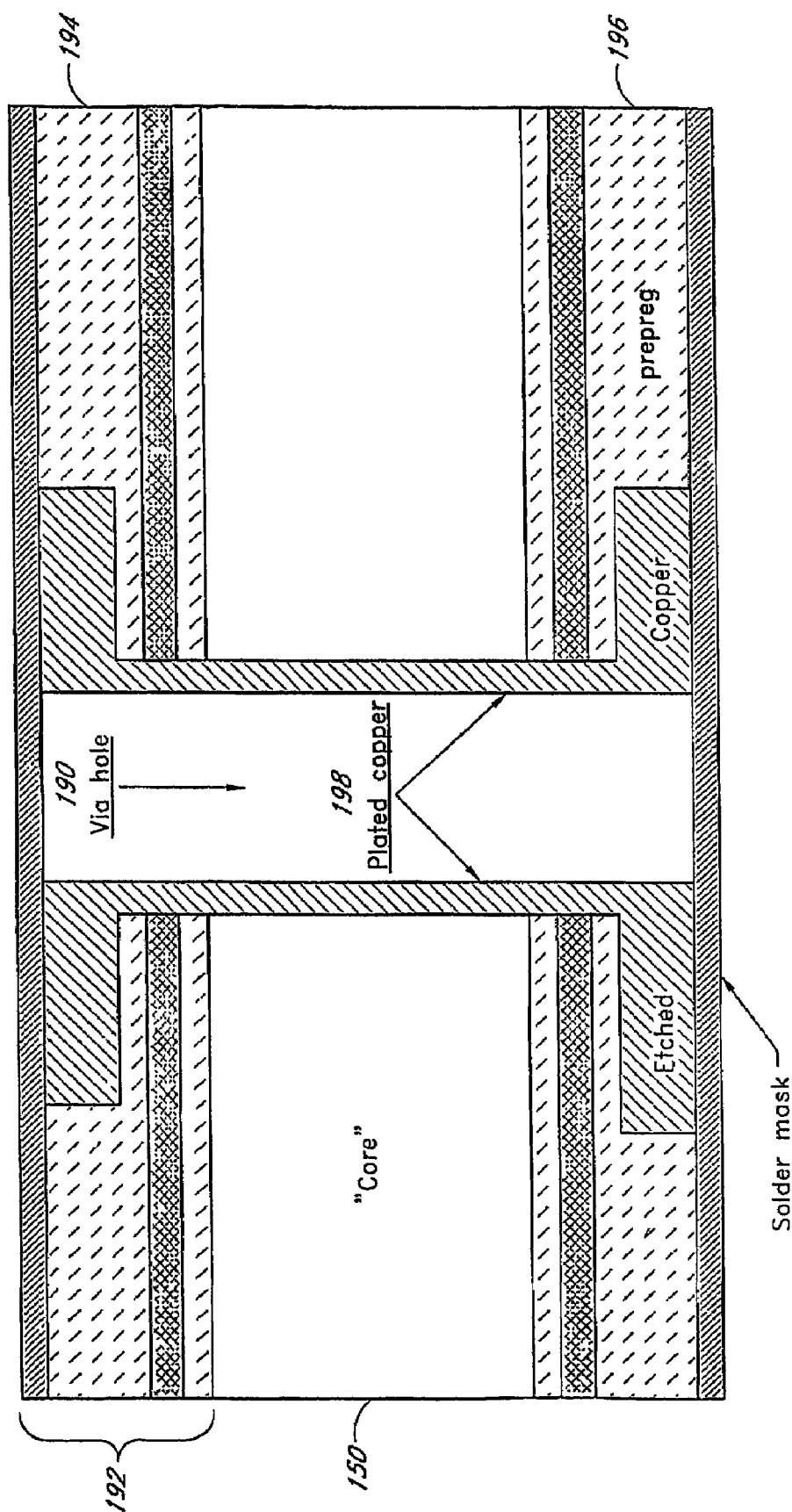
Cross section of via hole
