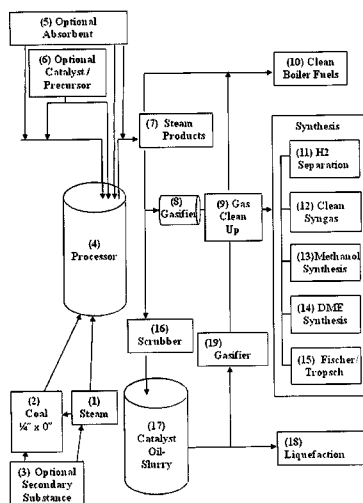
Overview of Products and Processes in Illustrative In-Line Configuration
