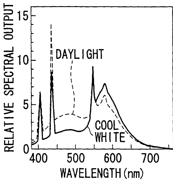
COOL WHITE AND DAYLIGHT FLUORESCENT LAMP
