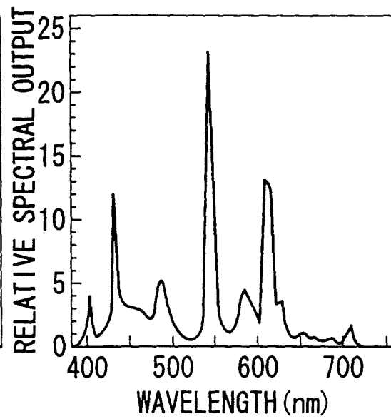
THREE WAVELENGTHS FLUORESCENT LAMP
