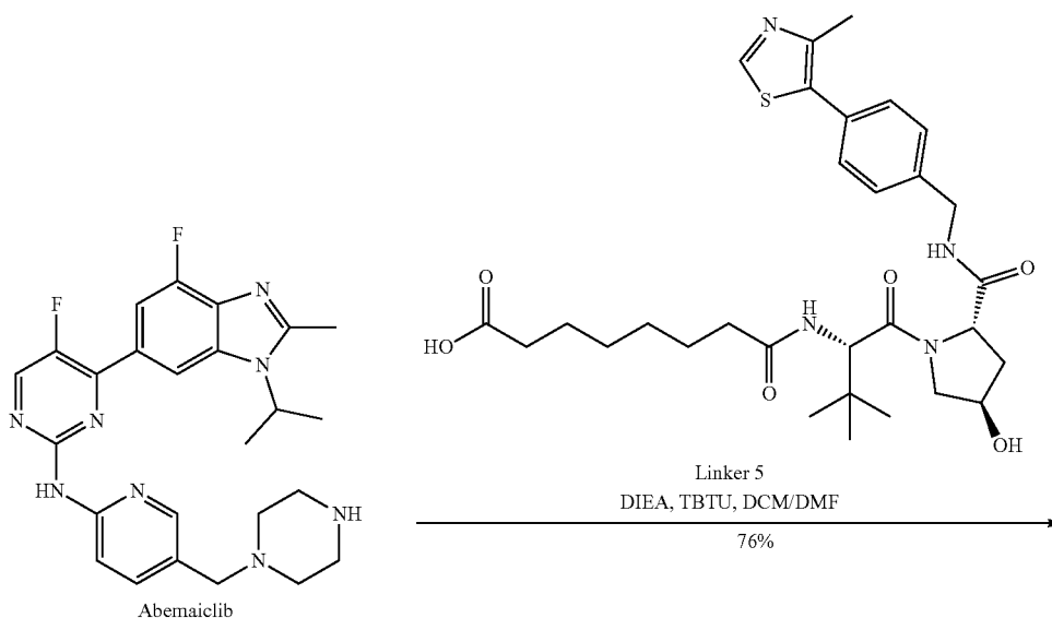
Scheme 8: Synthesis of example 32
