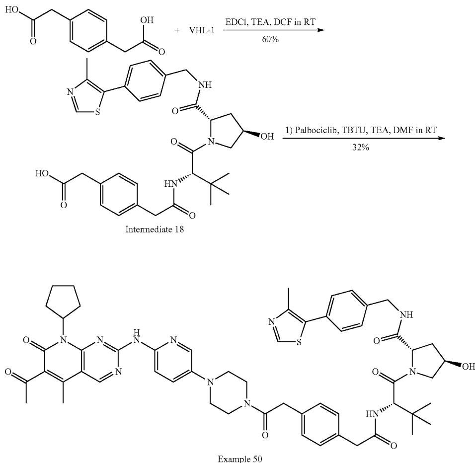
Scheme 21: Synthesis of example 50
