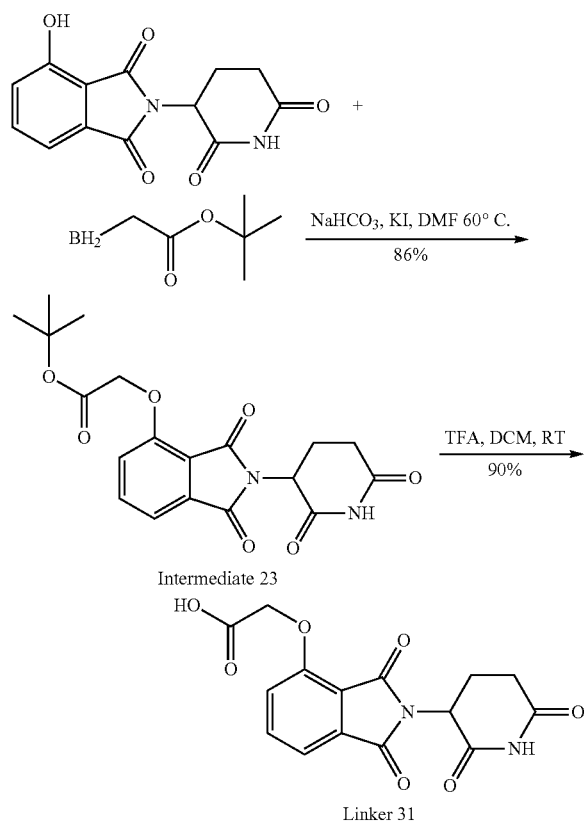
Scheme 26: Synthesis of Linker 31
