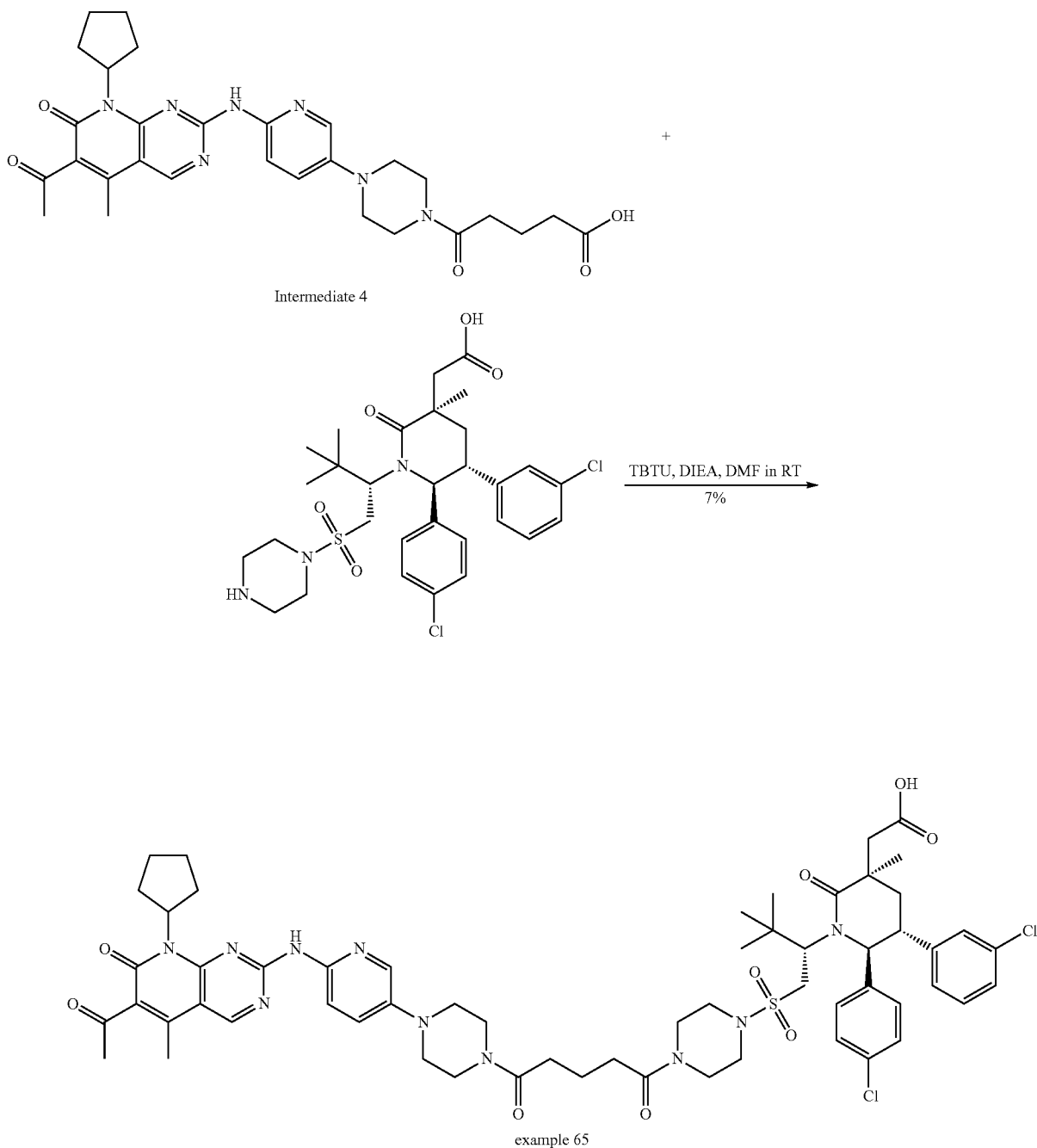
Scheme 33: synthesis of example 65
