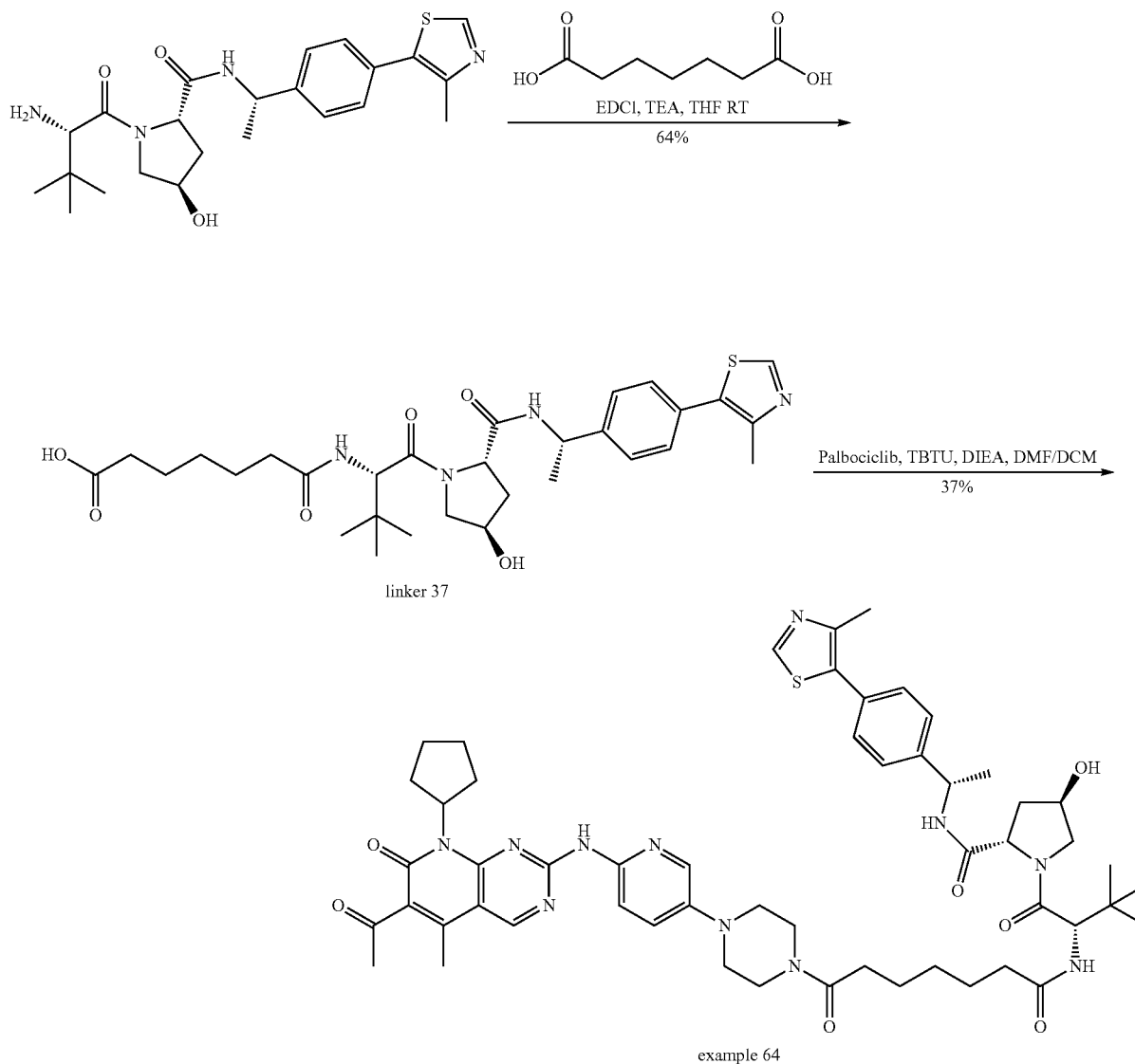
Scheme 32: synthesis of example 64
