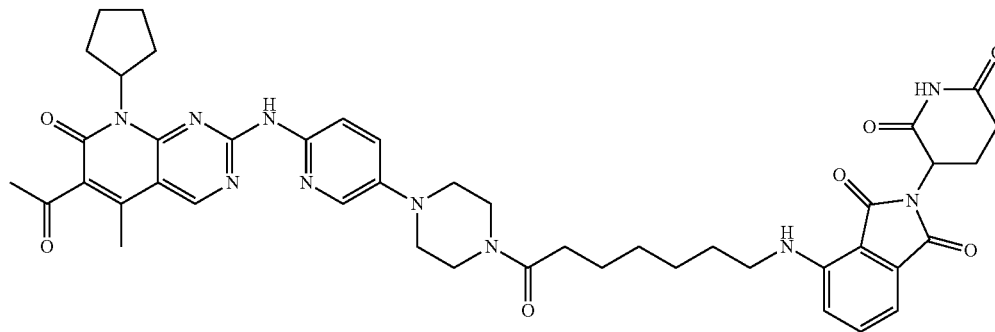
4-((7-(4-(6-((6-Acetyl-8-cyclopentyl-5-methyl-7-oxo-7,8-dihydropyrido[2,3-d]pyrimidin-2-yl)amino)pyridin-3-yl)piperazin-1-yl)-7-oxoheptyl)amino)-2-(2,6-dioxopiperidin-3-yl)isoindoline-1,3-dione (compound Example 28)
