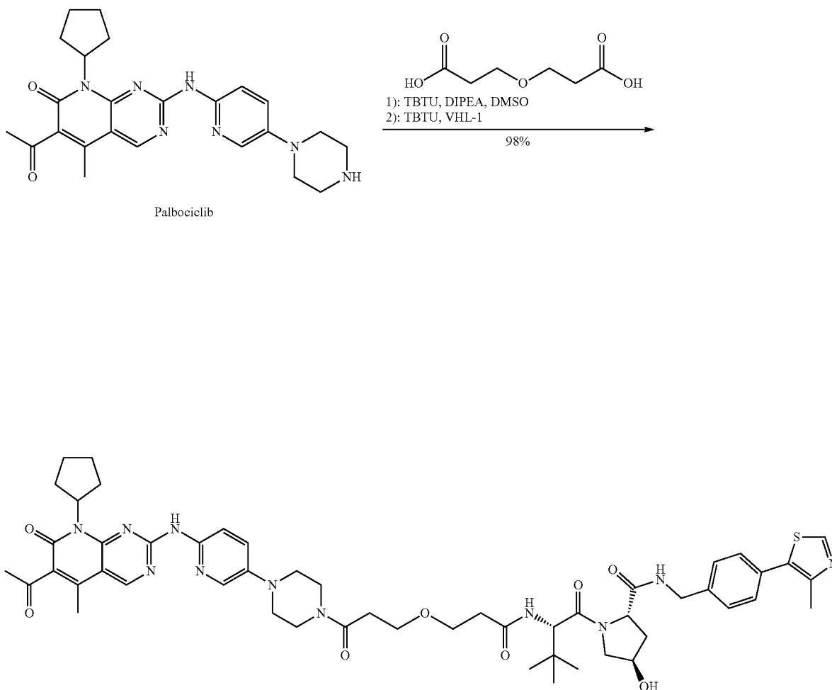
Scheme 2: Synthesis of example 2
