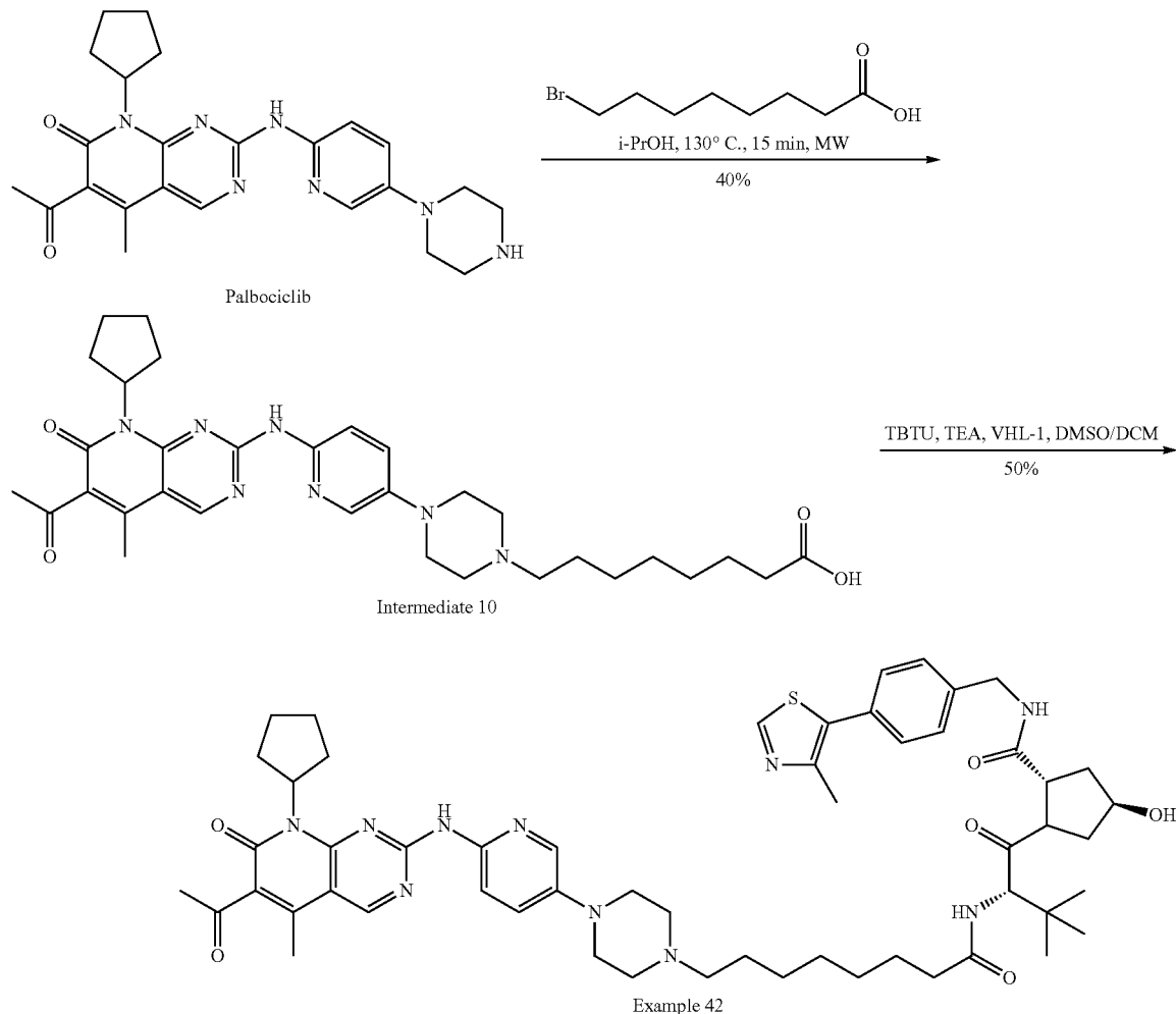
Scheme 14: Synthesis of example 42
