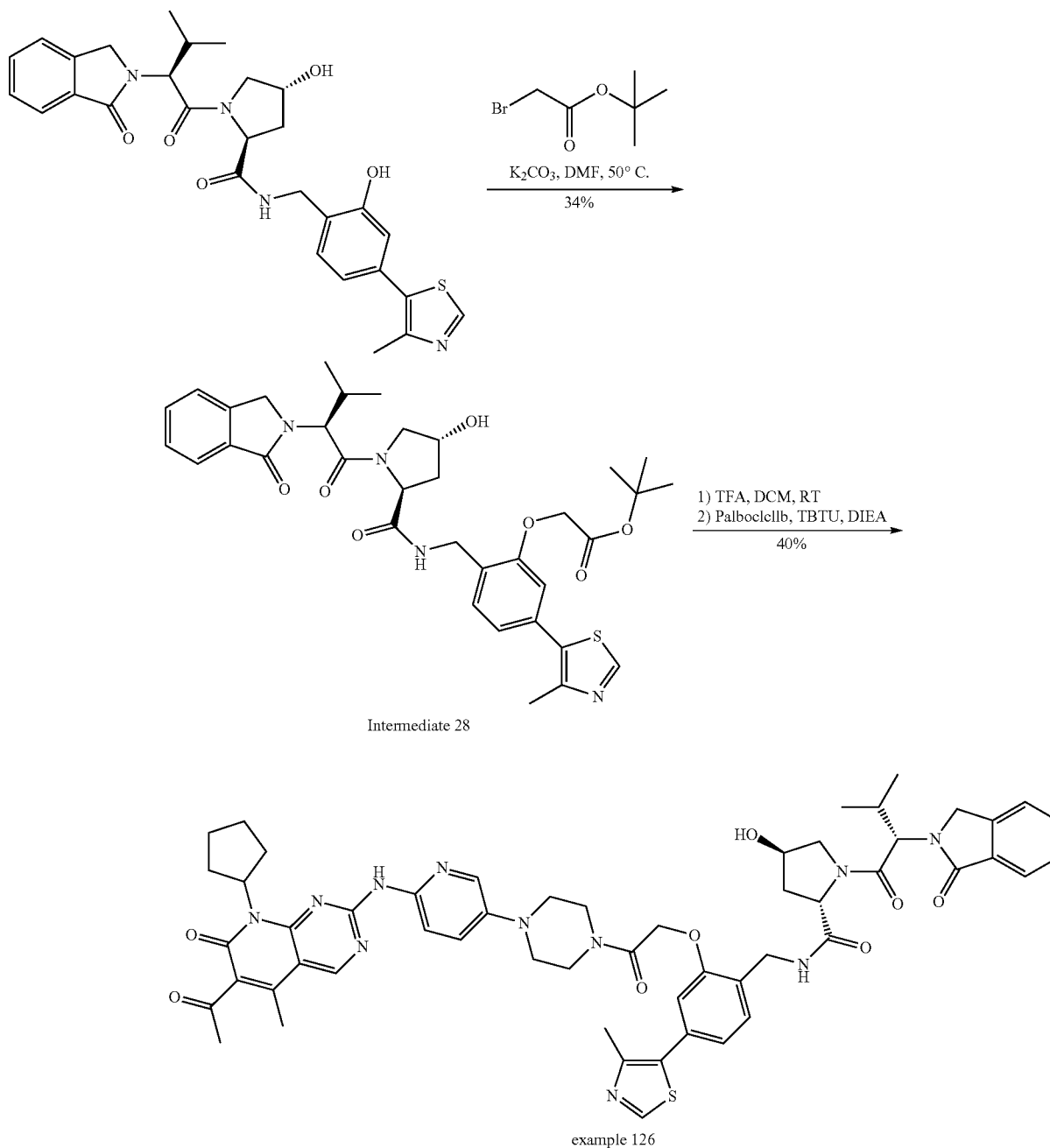
Scheme 36: synthesis of example 126
