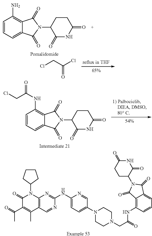
Scheme 24: Synthesis of example 53
