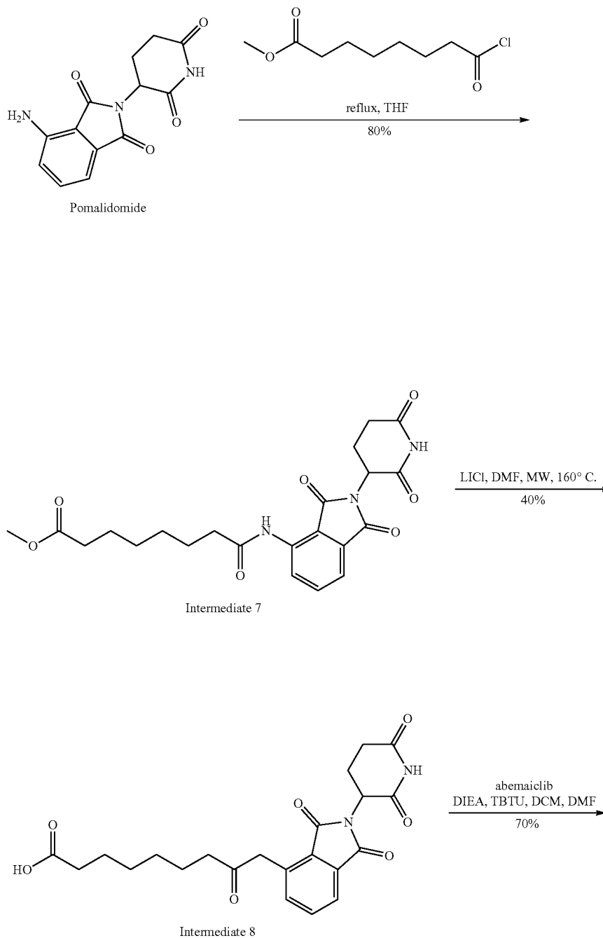
Scheme 7: Synthesis of example 31
