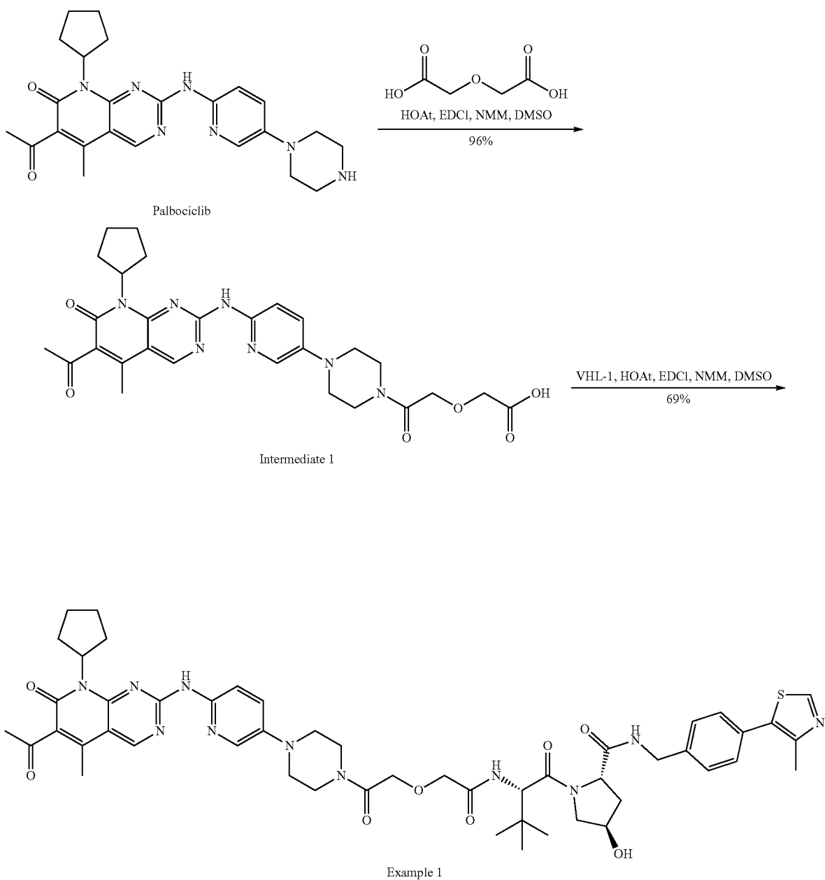
Scheme 1: Synthesis of example 1
