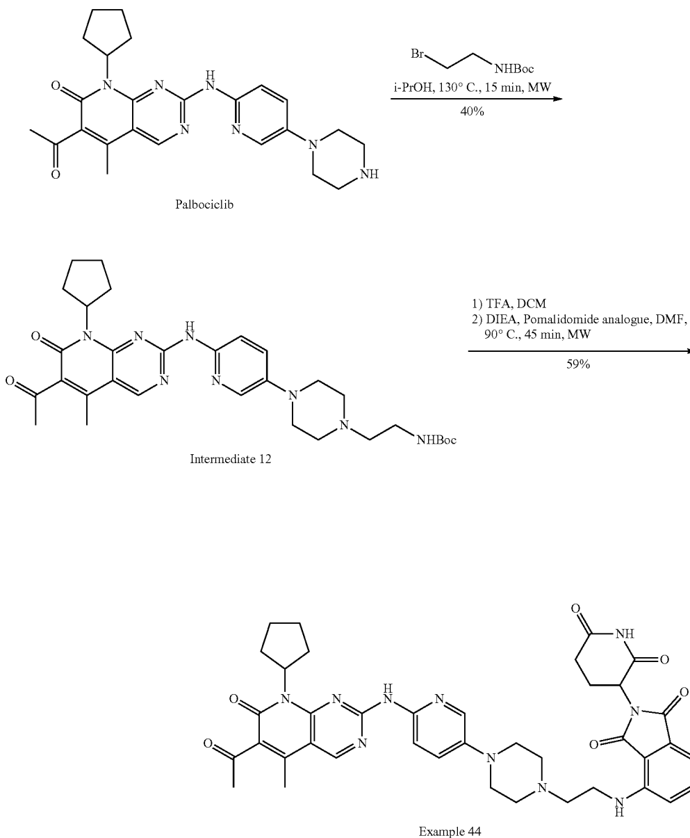
Scheme 16: Synthesis of example 44
