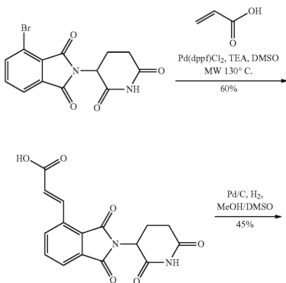
Scheme 31: Synthesis of Linker 36
