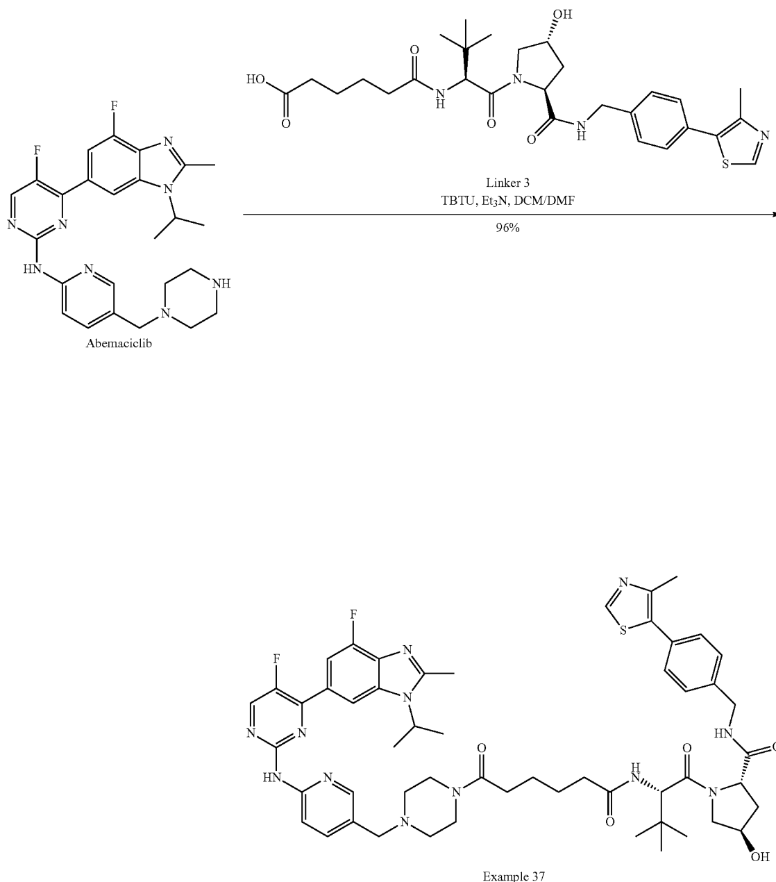
Scheme 10: synthesis of example 37
