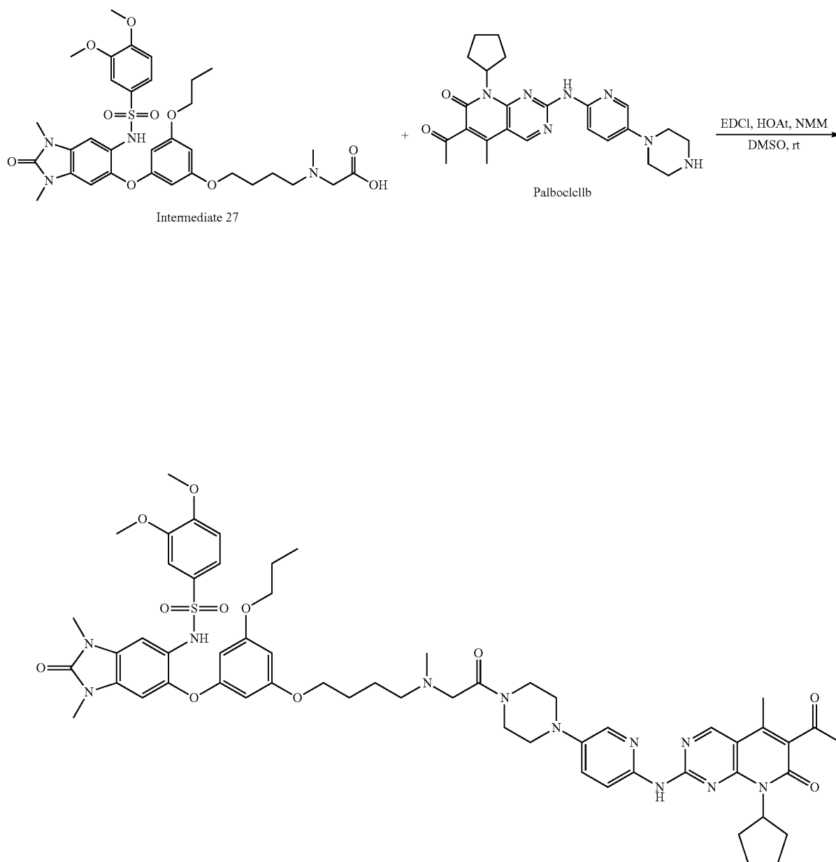
Scheme 35: synthesis of example 67
