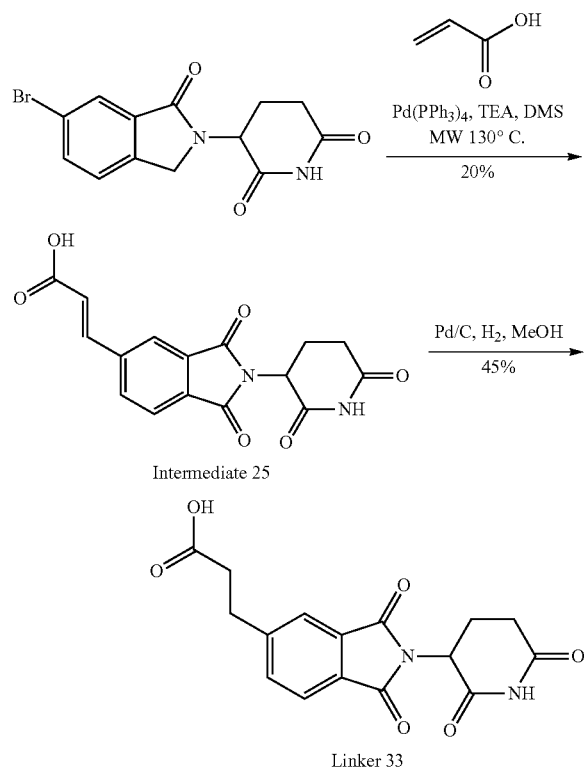
Scheme 28: Synthesis of Linker 33
