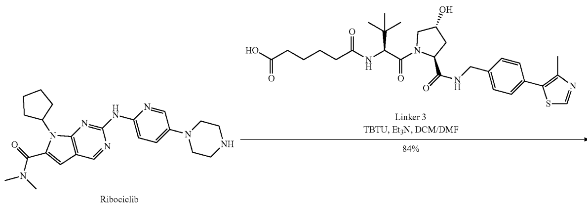
Scheme 9: synthesis of example 33
