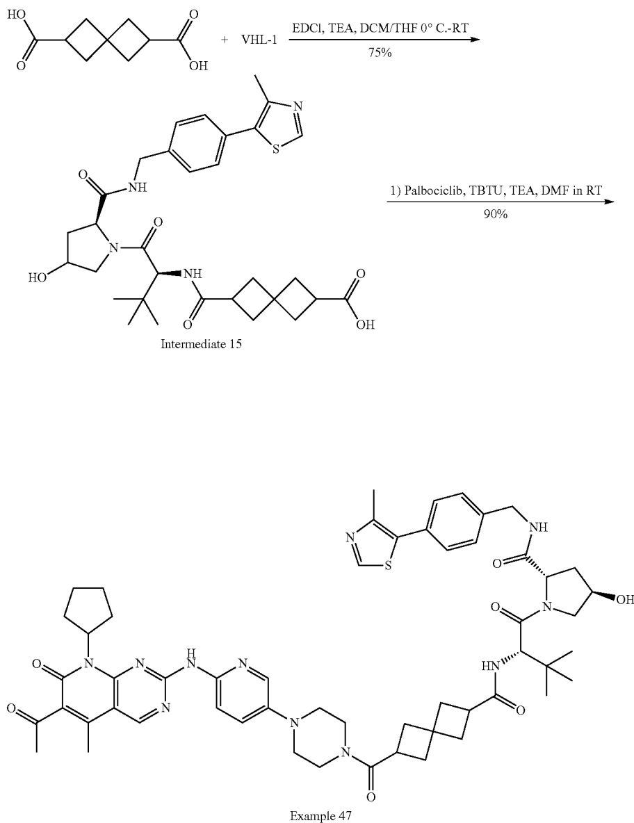
Scheme 18: Synthesis of example 47
