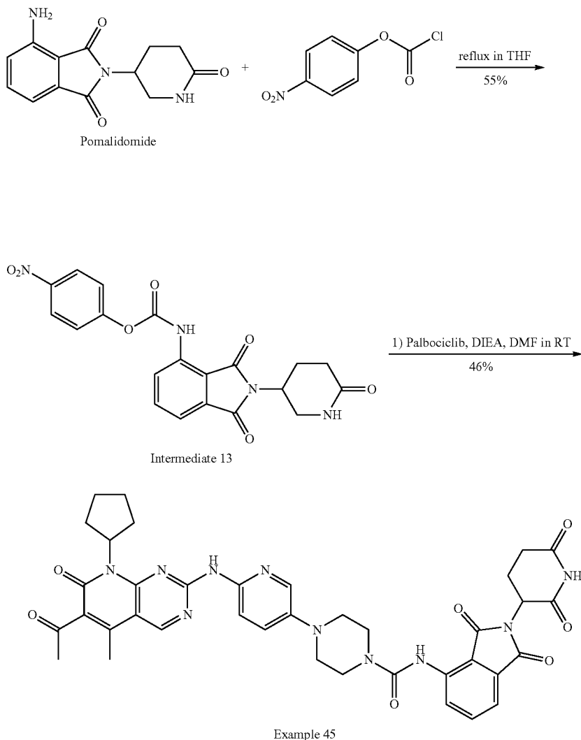
Scheme 17: Synthesis of example 45
