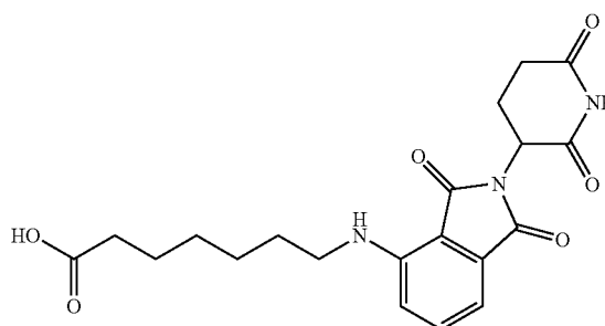
Linker 27: 7-((2-(2,6-Dioxopiperidin-3-yl)-1,3-dioxoisindolin-4-yl)amino)heptanoic acid
