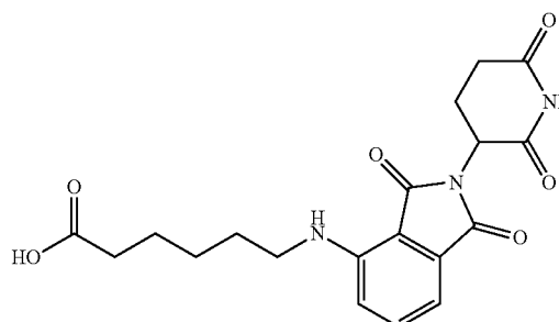
Linker 26: 6-((2-(2,6-Dioxopiperidin-3-yl)-1,3-dioxoisindolin-4-yl)amino)hexanoic acid
