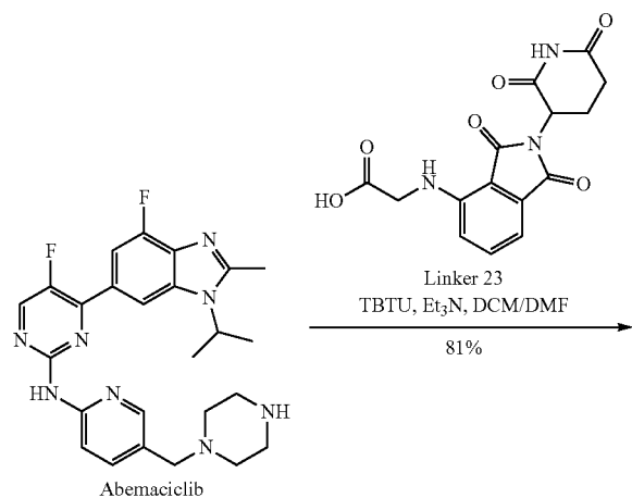
Scheme 12: synthesis of example 40
