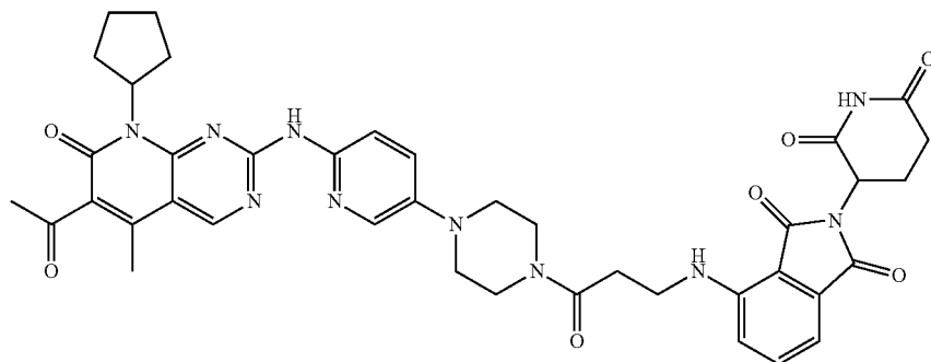
4-((3-(4-(6-((6-Acetyl-8-cyclopentyl-5-methyl-7-oxo-7,8-dihydropyrido[2,3-d]pyrimidin-2-yl)amino)pyridin-3-yl)piperazin-1-yl)-3-oxopropyl)amino)-2-(2,6-dioxopiperidin-3-yl)isoindoline-1,3-dione (compound Example 25) 20
