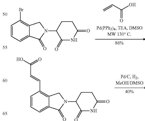
Scheme 30: Synthesis of Linker 35
