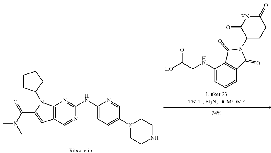
Scheme 11: synthesis of example 39
