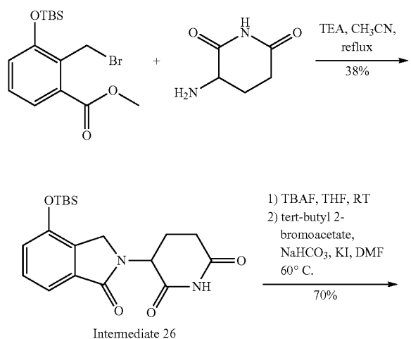
Scheme 29: Synthesis of Linker 34
