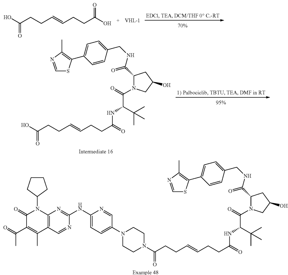
Scheme 19: Synthesis of example 48
