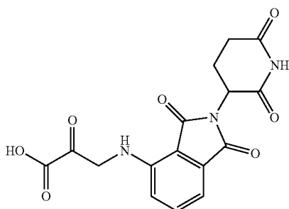
Linker 24: 3-((2-(2,6-Dioxopiperidin-3-yl)-1,3-dioxoisindolin-4-yl)amino)propanoic acid
