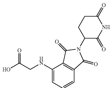
Linker 23: (2-(2,6-Dioxopiperidin-3-yl)-1,3-dioxoisindolin-4-yl)glycine
