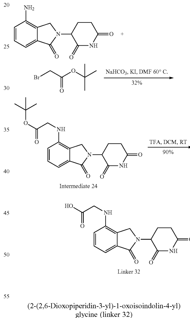
Scheme 27: Synthesis of Linker 32
