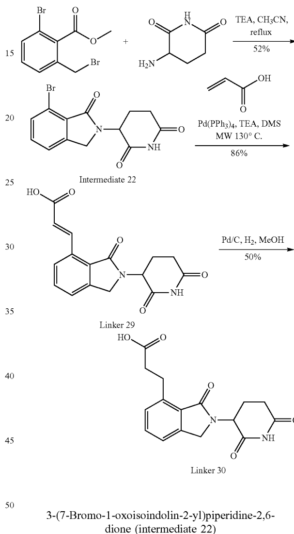
Scheme 25: Synthesis of Linker 29 and 30
