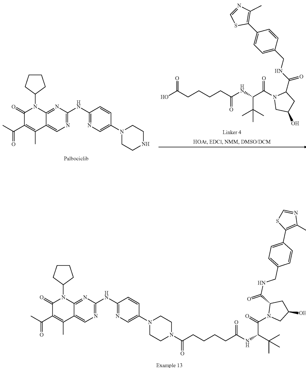
Scheme 4: Synthesis of example 13
