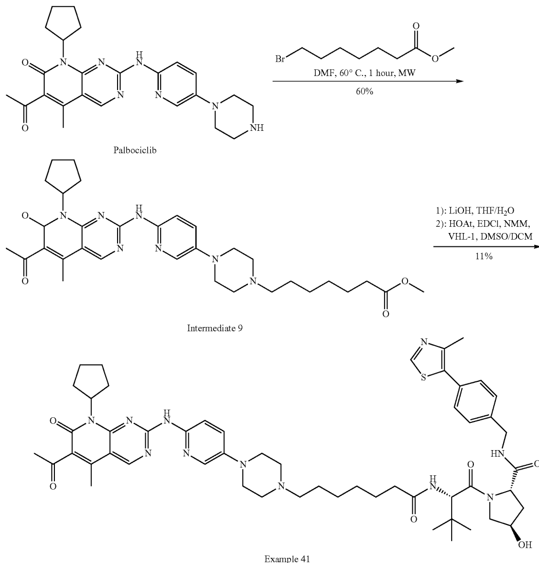
Scheme 13: Synthesis of example 41
