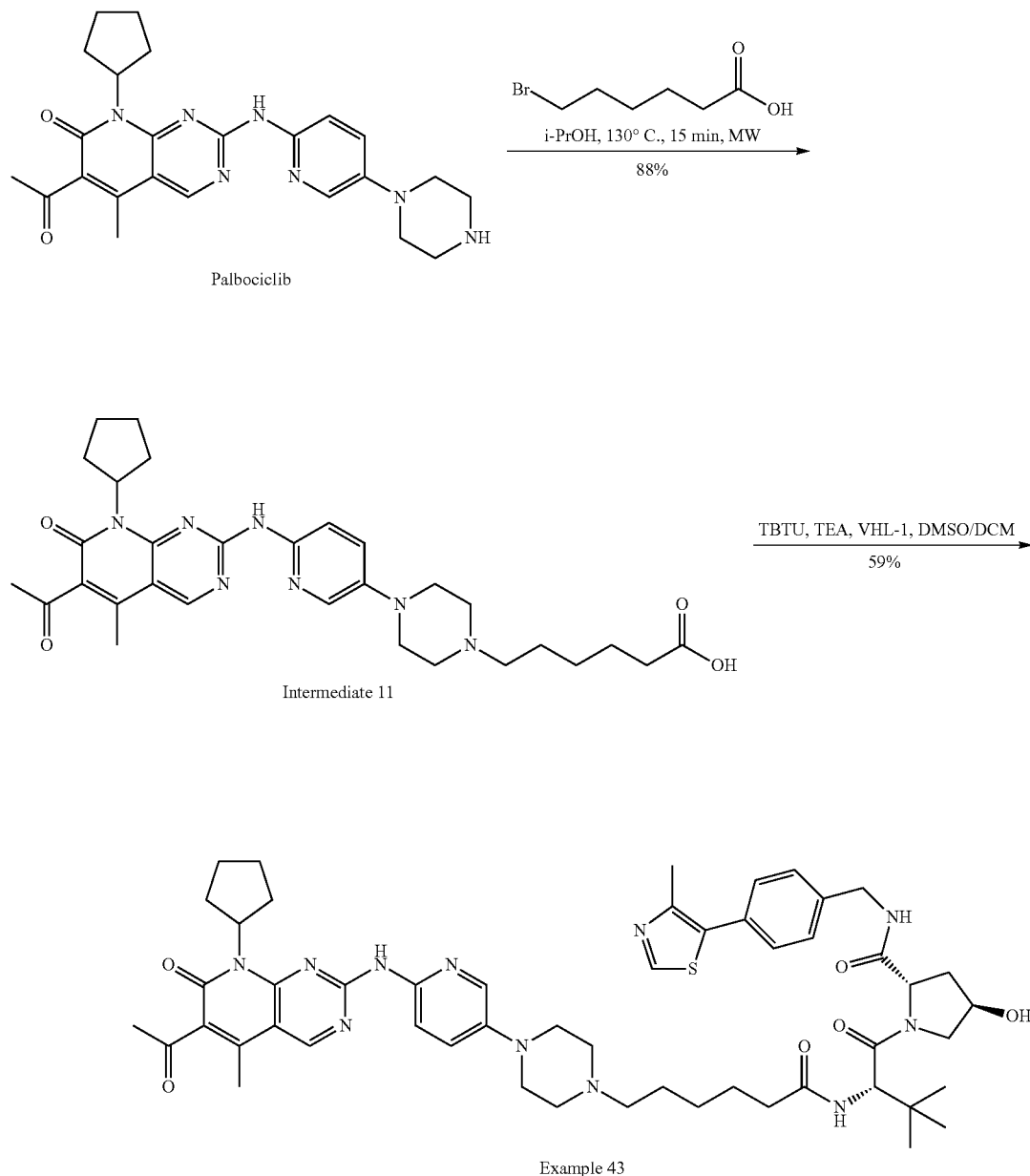
Scheme 15: Synthesis of example 43
