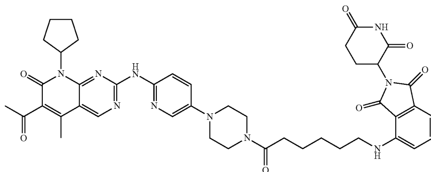
4-((6-(4-(6-((6-Acetyl-8-cyclopentyl-5-methyl-7-oxo-7,8-dihydropyrido[2,3-d]pyrimidin-2-yl)amino)pyridin-3-yl)piperazin-1-yl)-6-oxoheptyl)amino)-2-(2,6-dioxopiperidin-3-yl)isoindoline-1,3-dione (compound Example 27)
