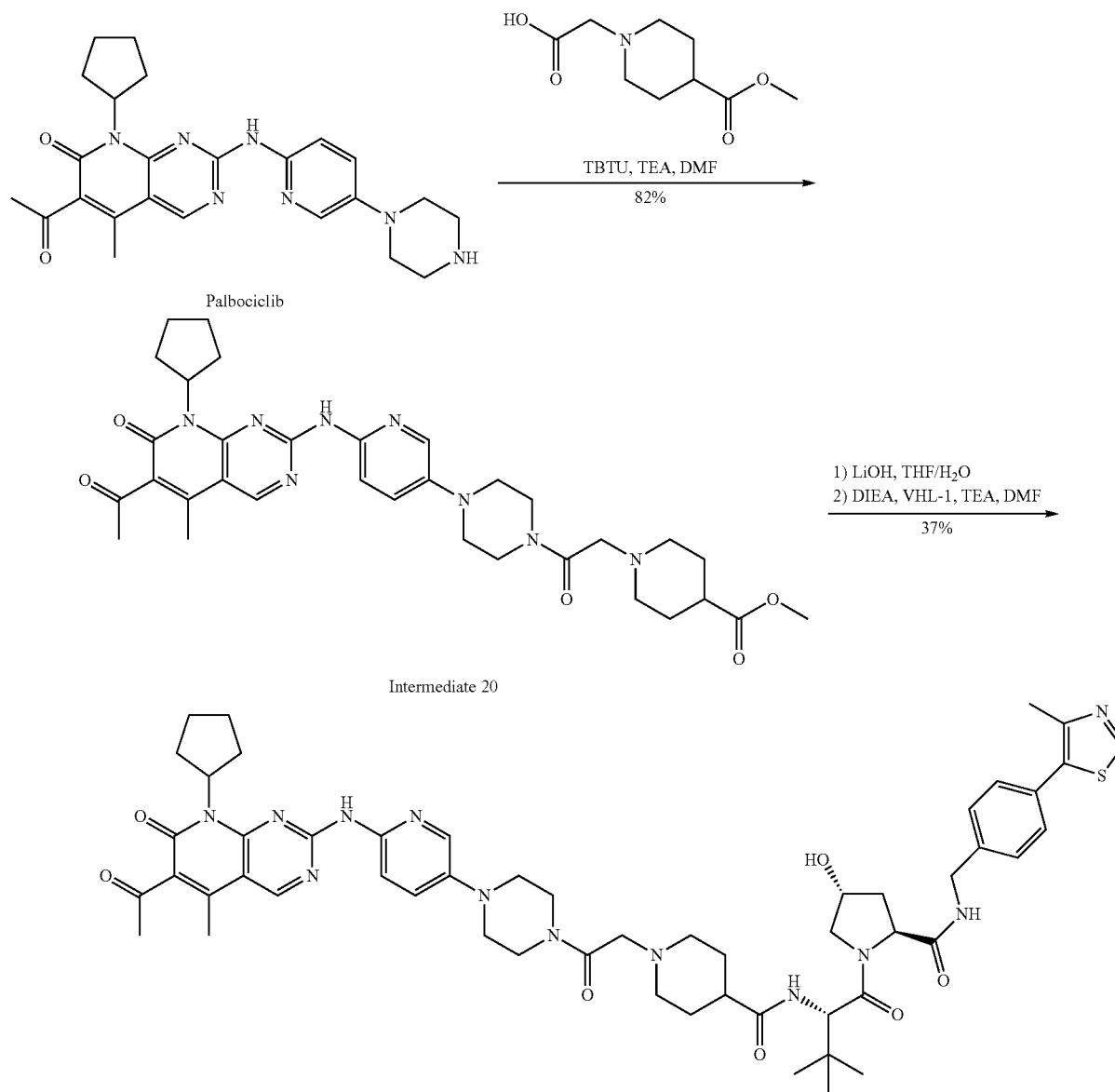
Scheme 23: Synthesis of example 52
