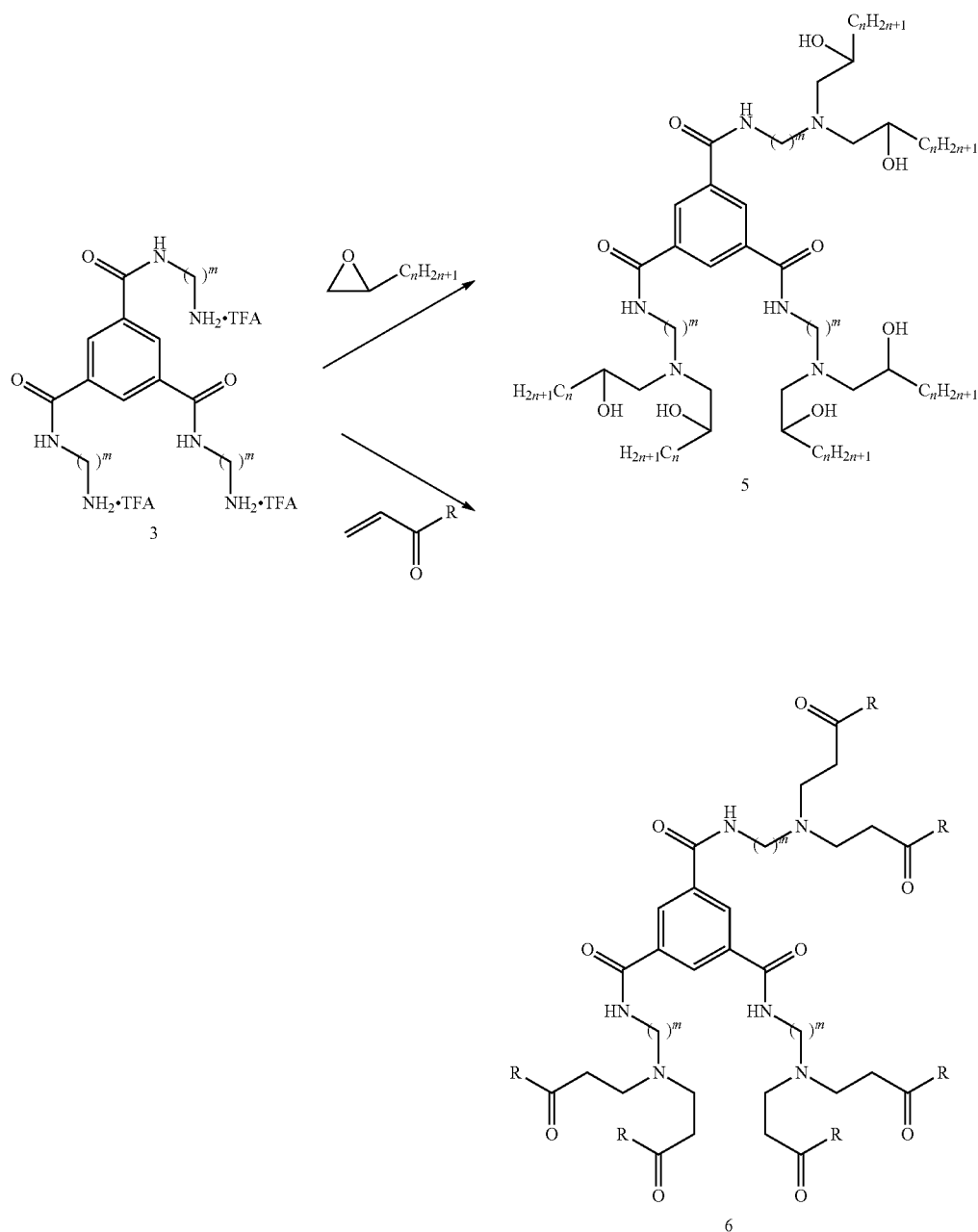
Scheme 5: Generic Synthetic Routes of Designed LLN
