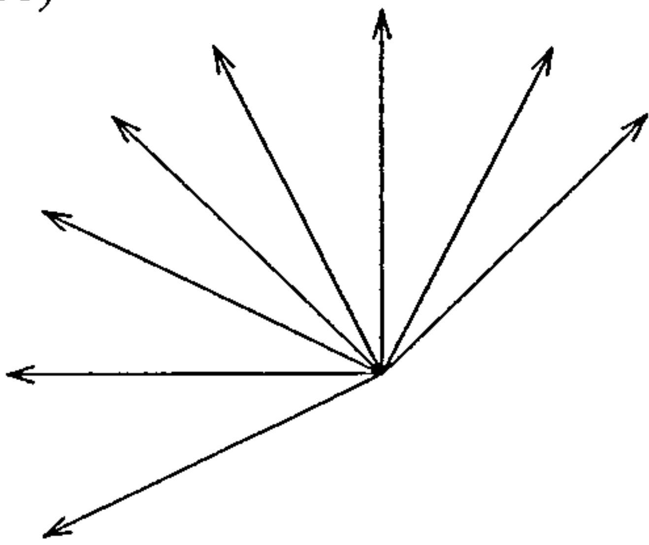
Directional Predictions in Case of N=9 (8 Modes)
