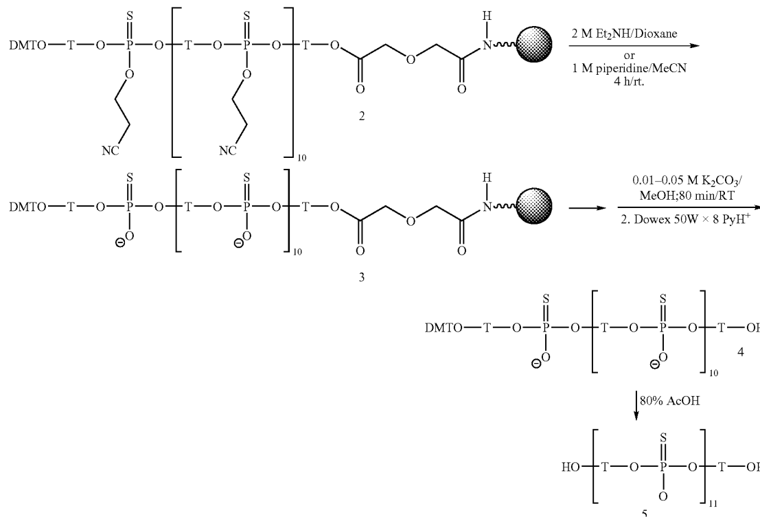
Scheme 2 Deprotection and releasing oligonucleotide 5 from solid support
