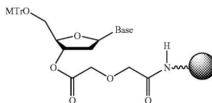
Scheme 1 Solid Supports
