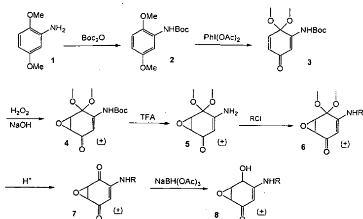
Reaction Scheme 1
