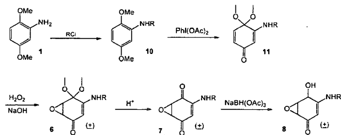
Reaction Scheme 2
