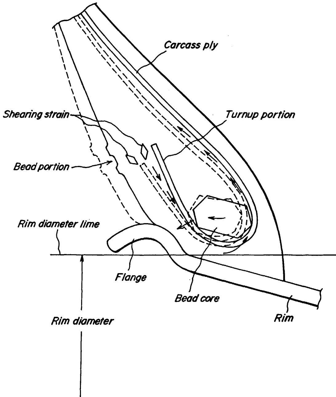
FIG. 22 PRIOR ART
