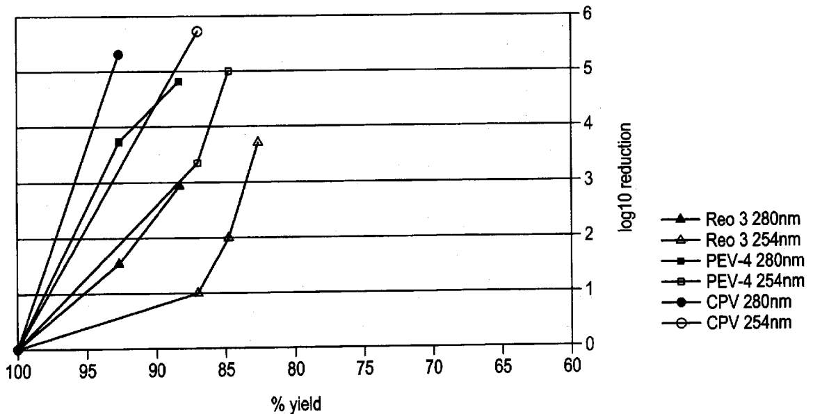
Comparison of inactivating various viruses by UV light of 254 nm and 280 nm in a factor VIII preparation
