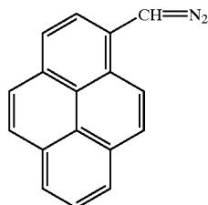
1-Pyrenyldiazomethane
