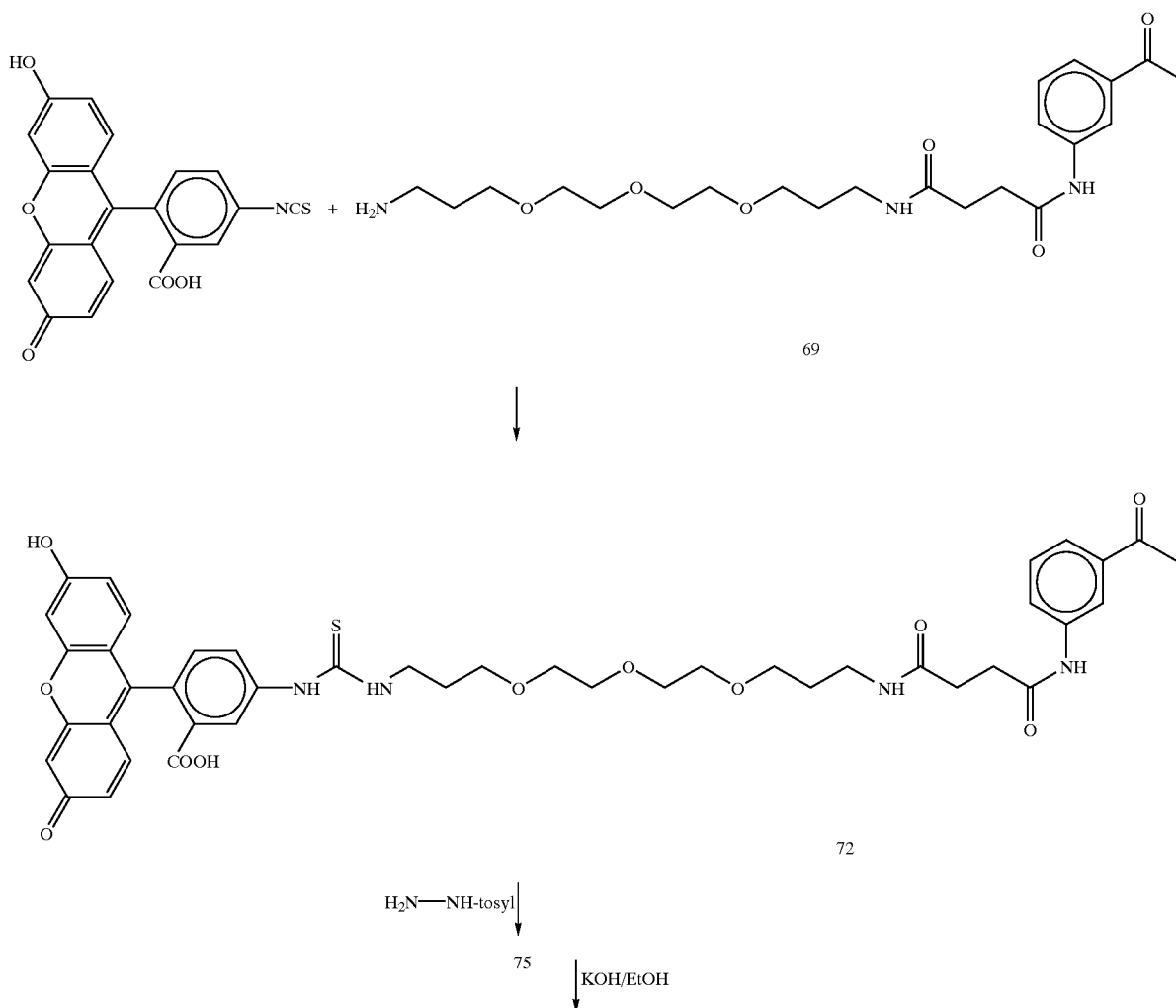
Synthesis scheme
