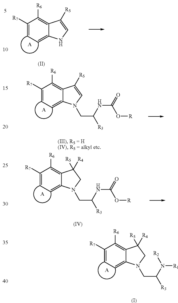
Reaction Scheme 1
