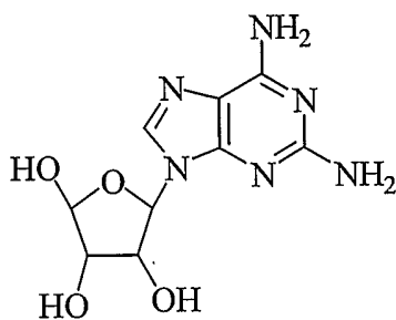
2,6-DiaminoPurine
