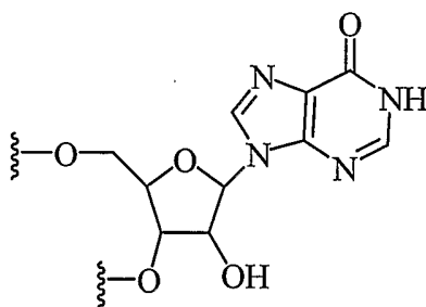
Inosine (I)
