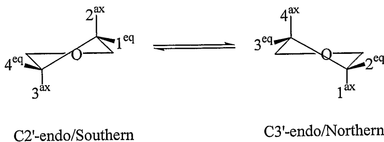
Conformation Scheme
