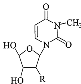
N3-methyl Uridine
