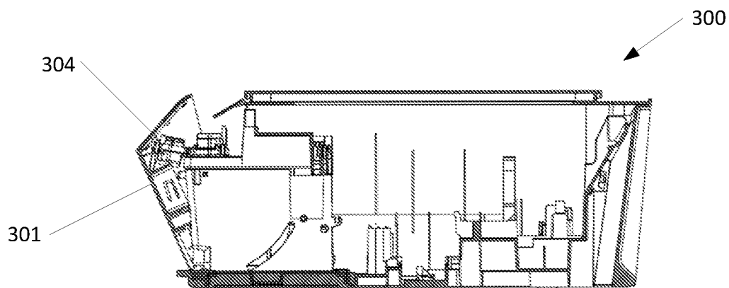
Figure 17 (section A-A)
