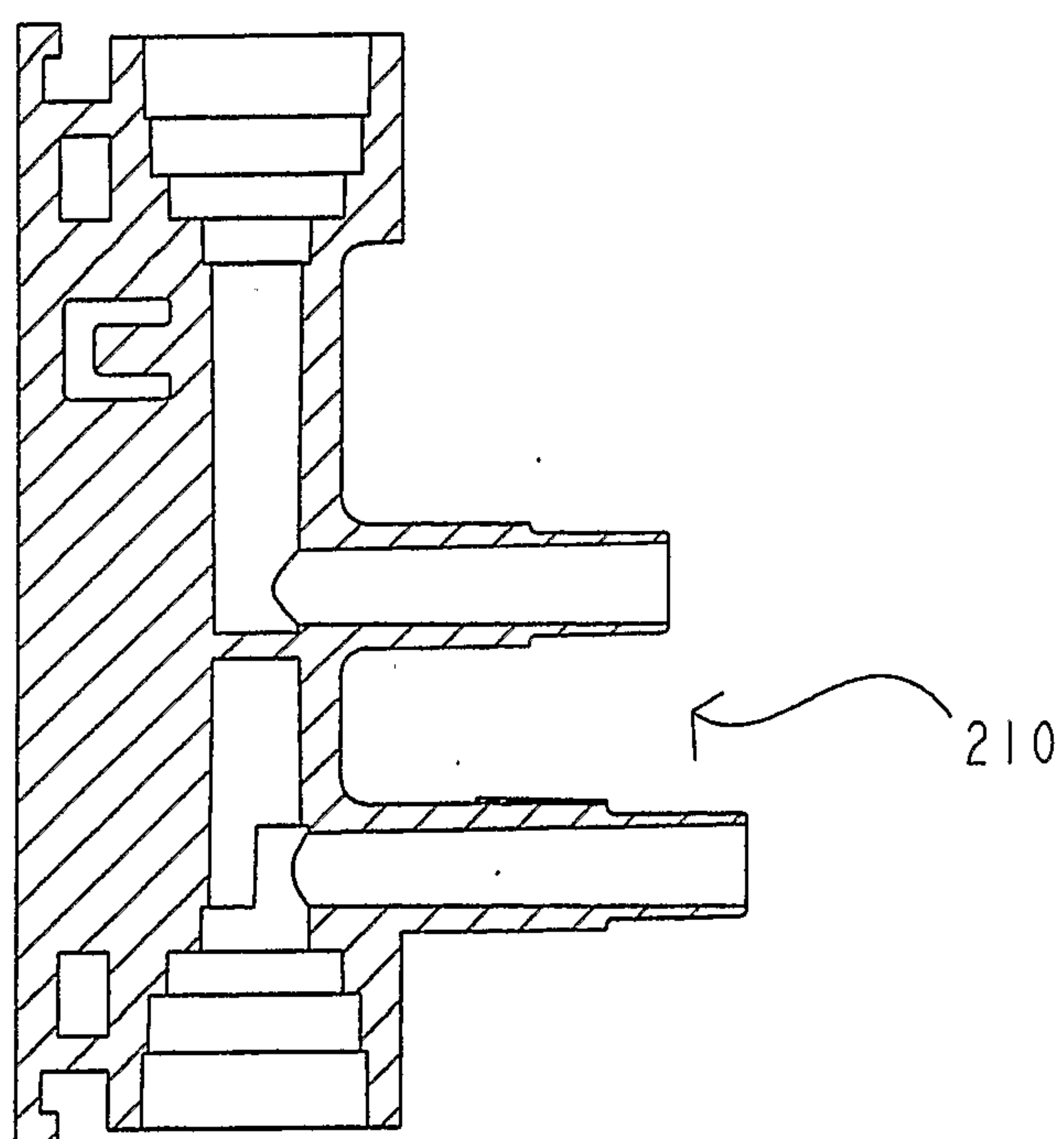
SECTION B-B
