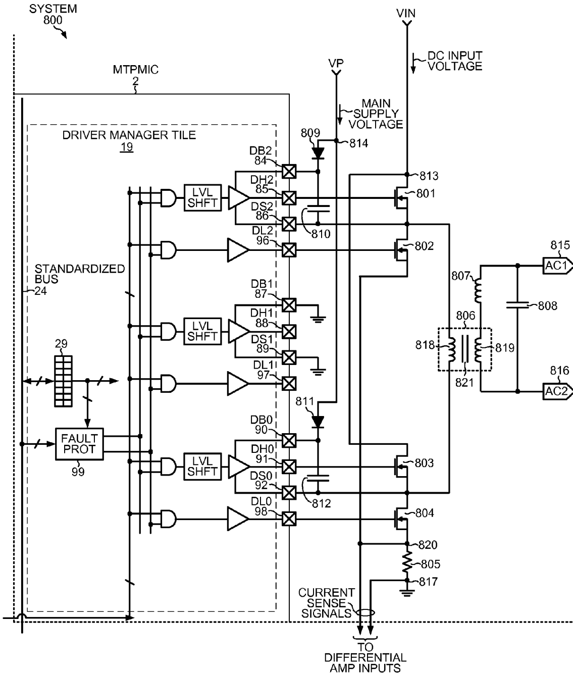
H-BRIDGE INVERTER FOR BACKUP UPS
