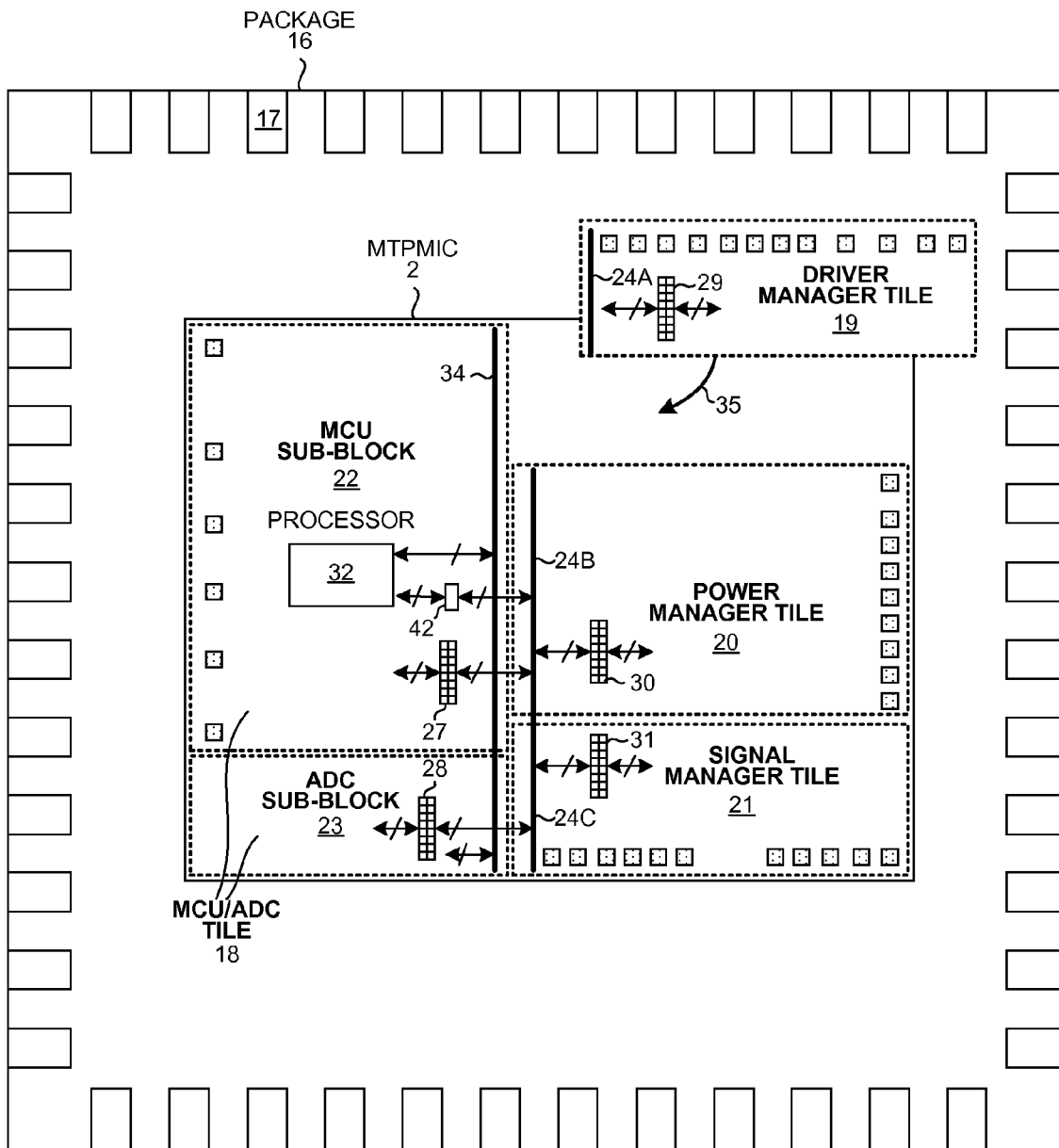
MTPMIC INTEGRATED CIRCUIT FIG. 2
