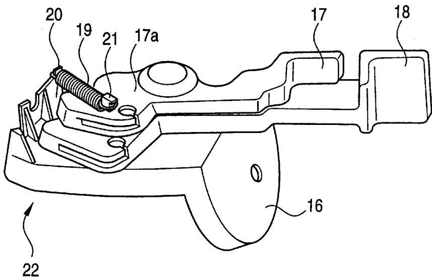
FIG. 6 (PRIOR ART)
