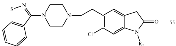
Formula XXI
