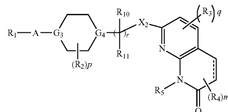
Formula XV
