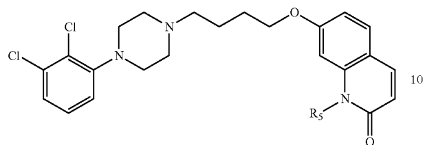
Formula XX 5
