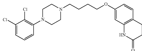
Aripiprazole
