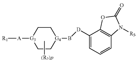
Formula XII
