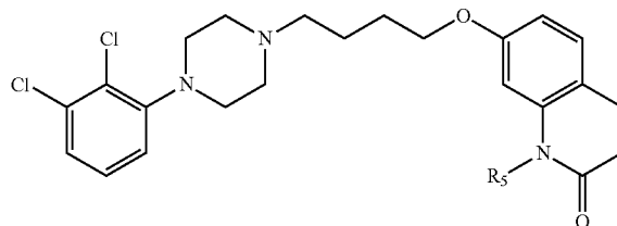
Formula XIX
