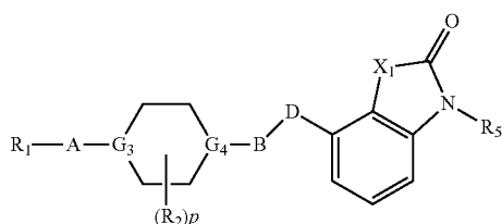
Formula XI
