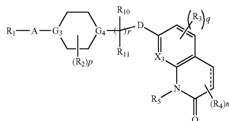
Formula XIV
