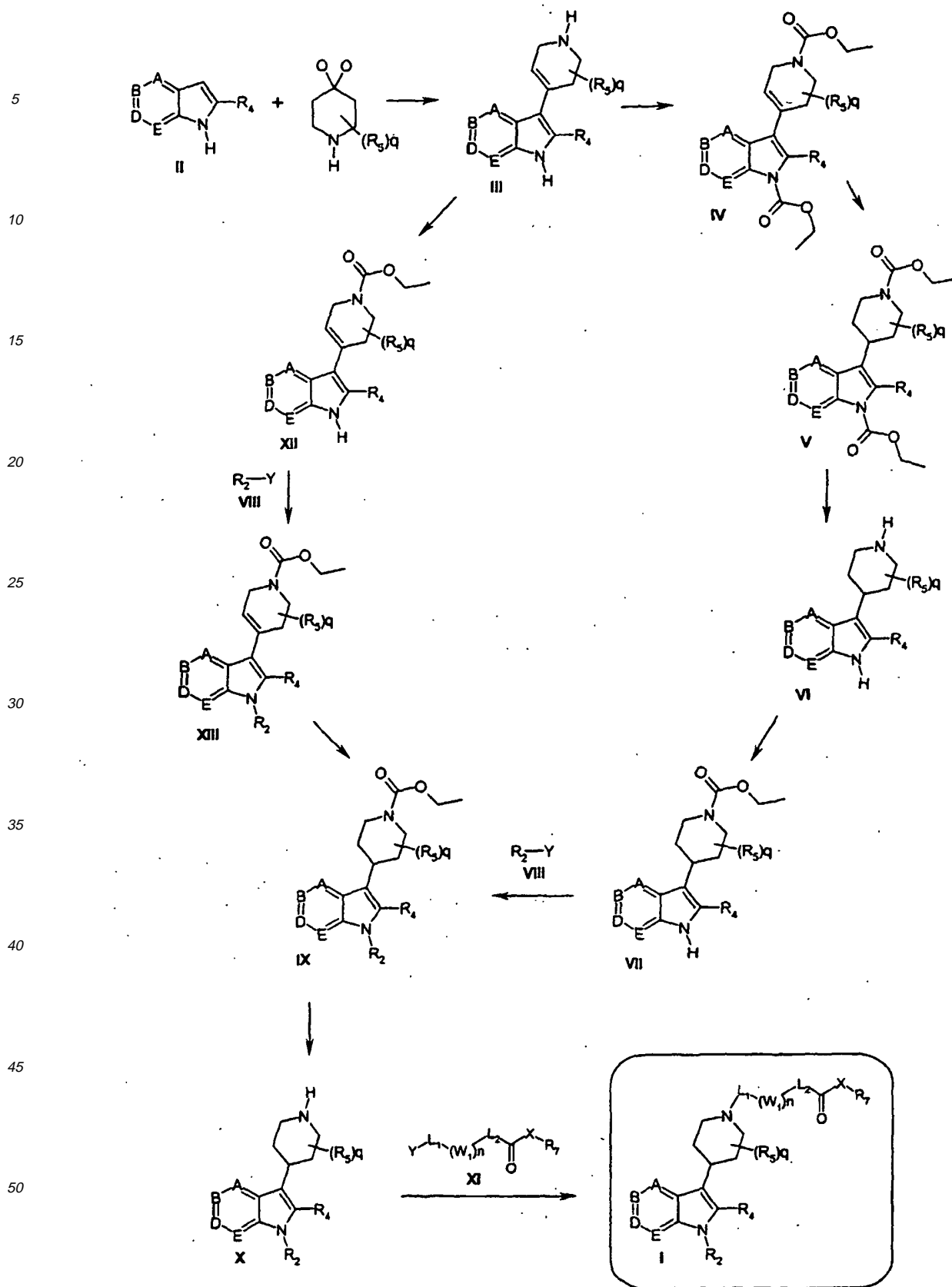
Scheme 1
