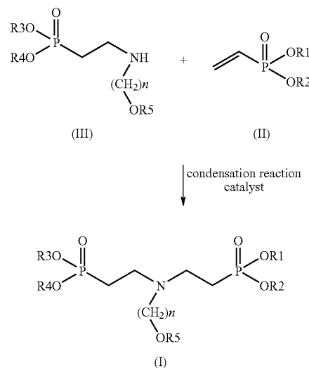
Reaction_Scheme_A
