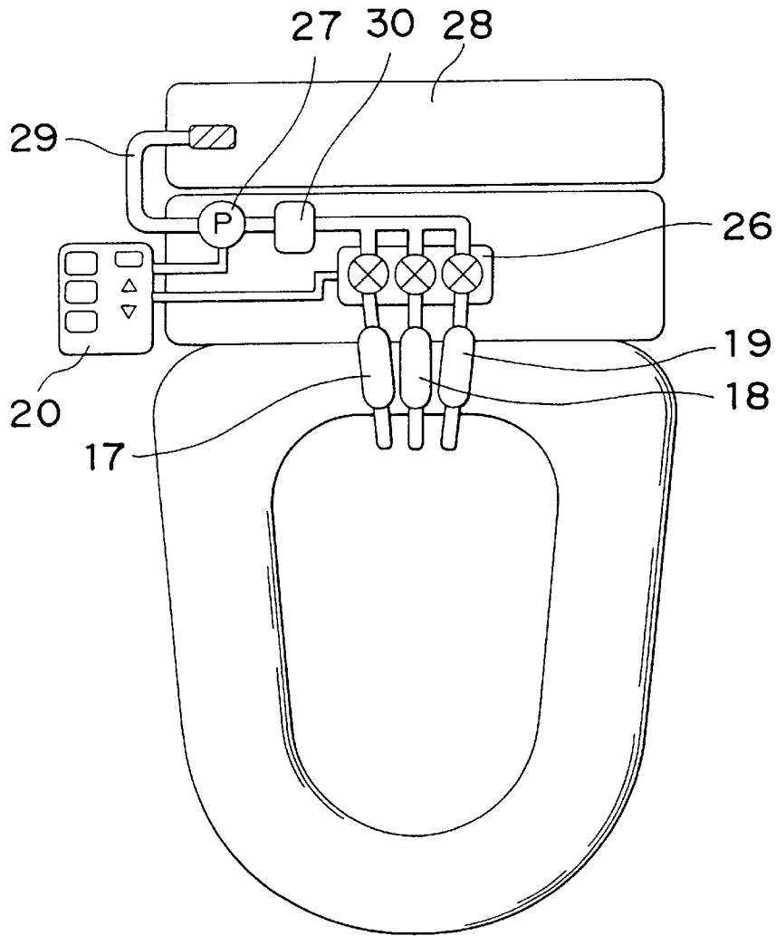
Fig. 3 PRIOR ART
