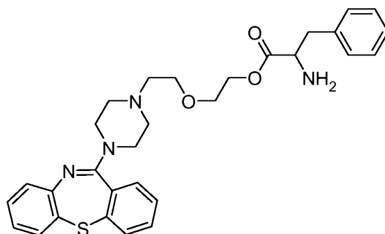
Phenylalanine-quetiapine (Phe-QTP)
