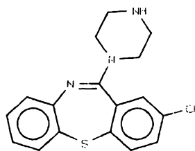
(2-Cl-norQTP),
