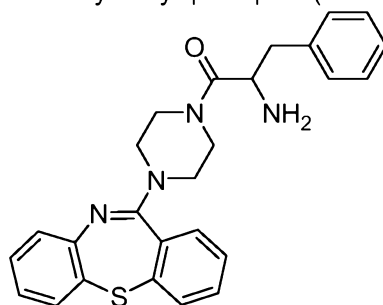
phenylalanine-N-desalkyl-quetiapine (Phe-norQTP)
