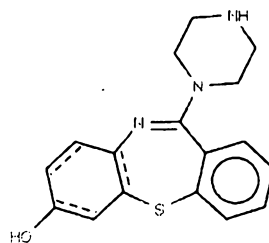
(7-OH-norQTP)
