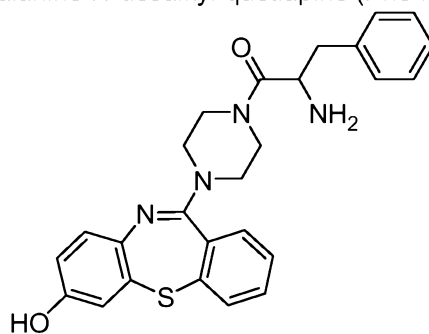
phenylalanine-7-hydroxy-N-desalkyl-quetiapine (Phe-7-OH-norQTP)
