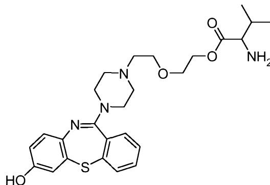
valine-7-hydroxy-quetiapine (Val-7-OH-QTP)
