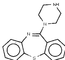
(norQTP),
