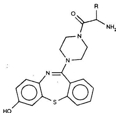
(X)
