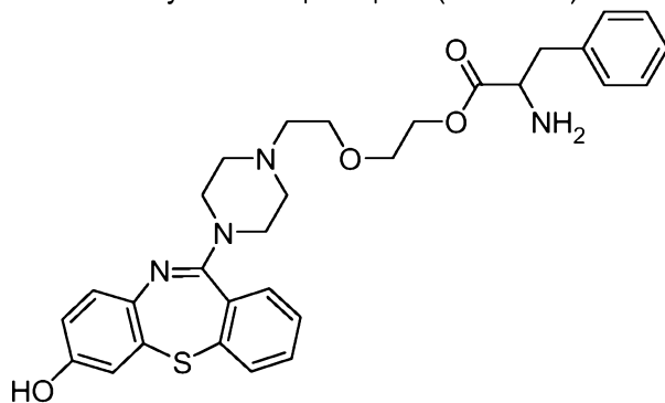
phenylalanine-7-hydroxy-quetiapine (Phe-7-OH-QTP)
