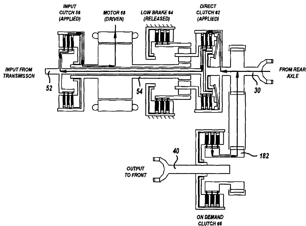
POWER FLOW FOR REGEN BRAKING (DIRECT MODE)
