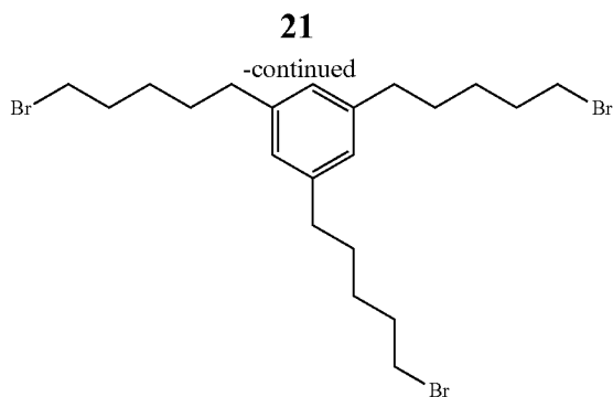
Preparation of 1,3,5-tris-(5-bromopentyl)-benzene
