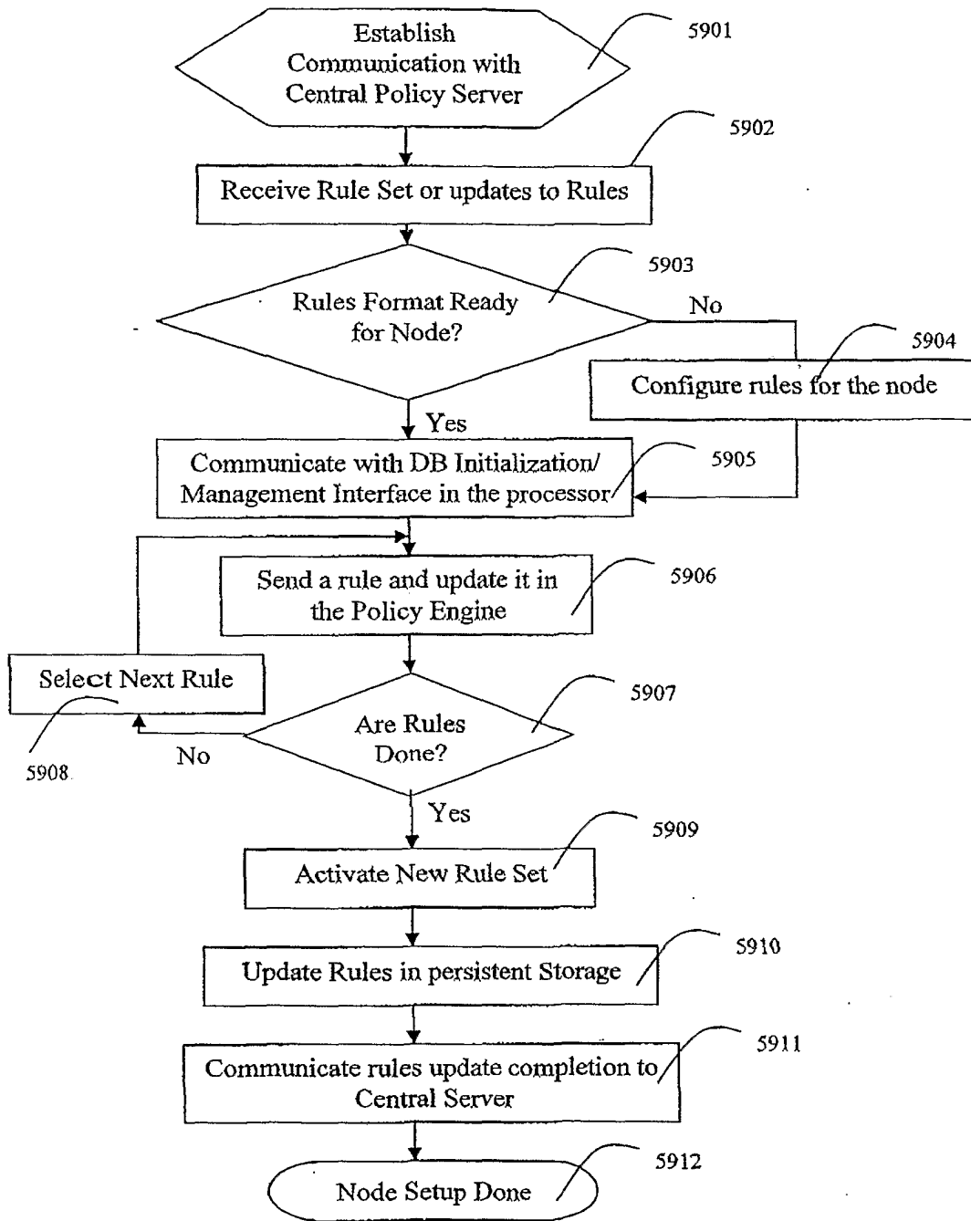
Fig. 59 Control Plane Processor/Policy Driver Flow
