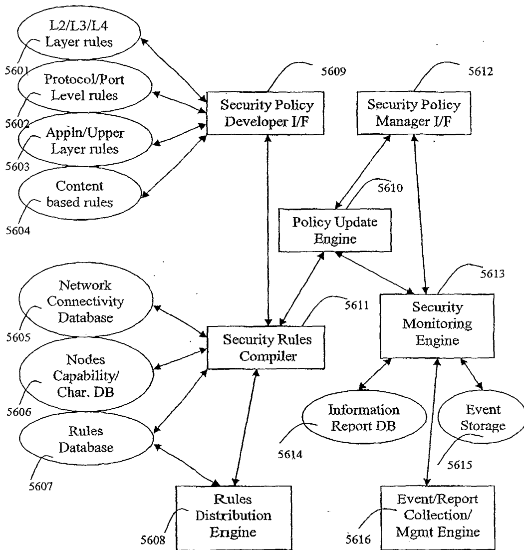
Fig. 56 Central Manager/Policy Server & Monitoring Station
