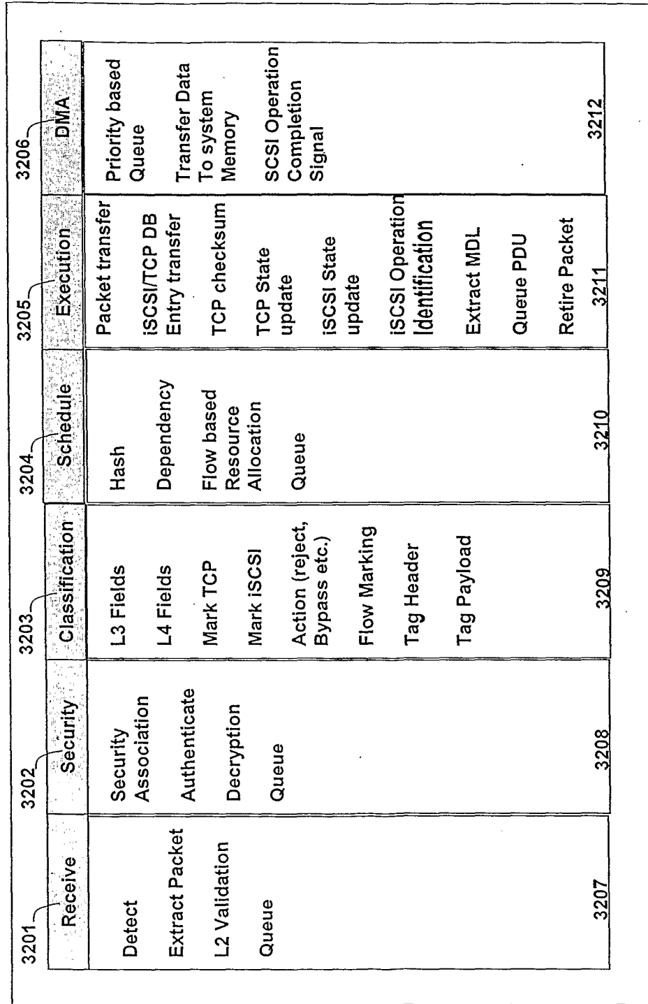
Fig. 32 Read Data Packet Flow
