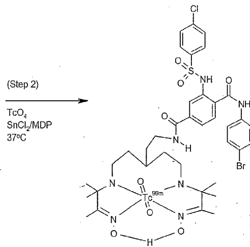
imaging agent 1
