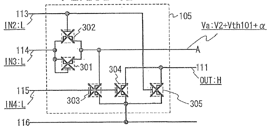
FIG. 12C PERIOD T2
