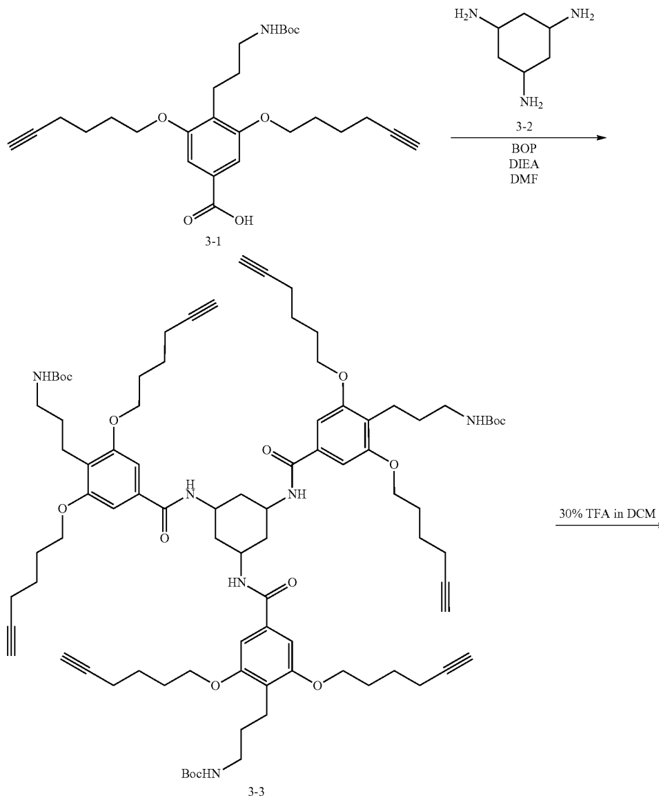
Scheme 20
