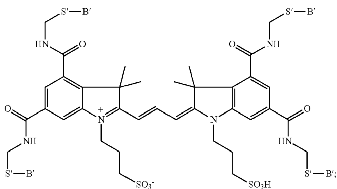
D010 (Tetravalent)
