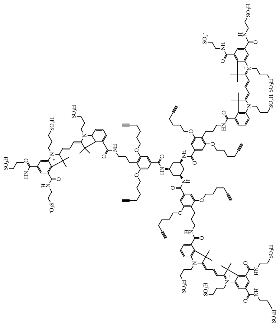
Scheme 5
