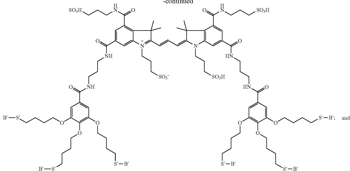
D009(PD-Gal) 2 (Hexavalent)
