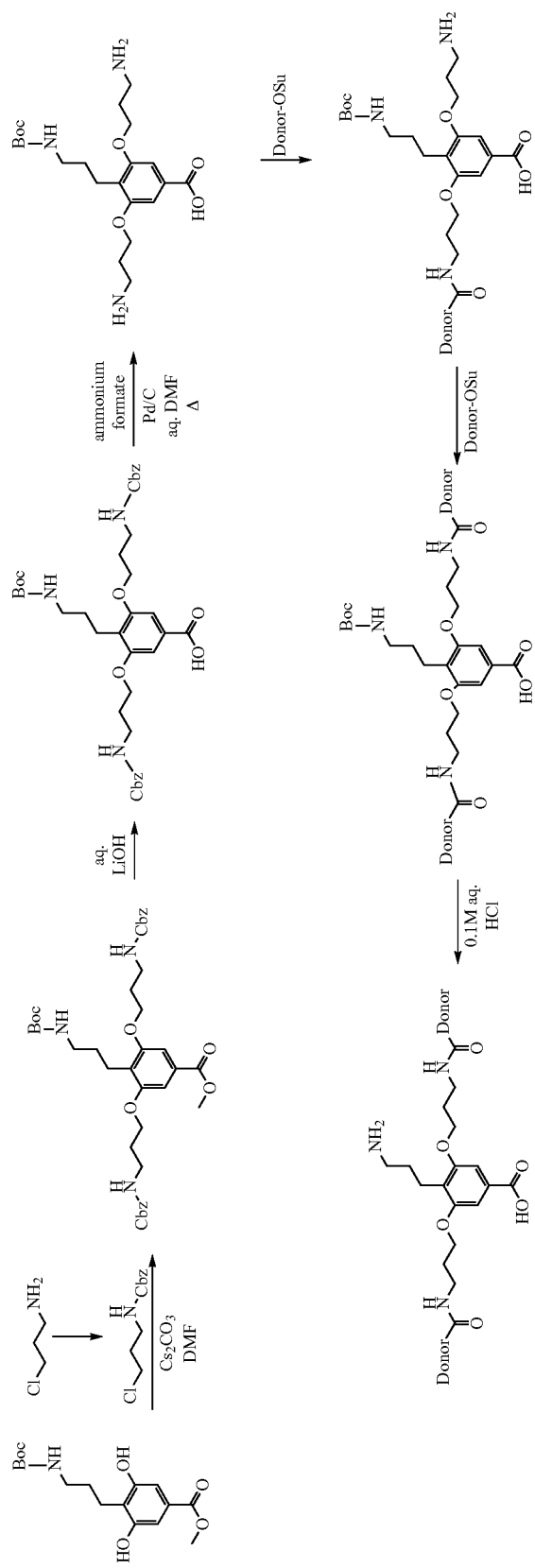
Scheme 9
