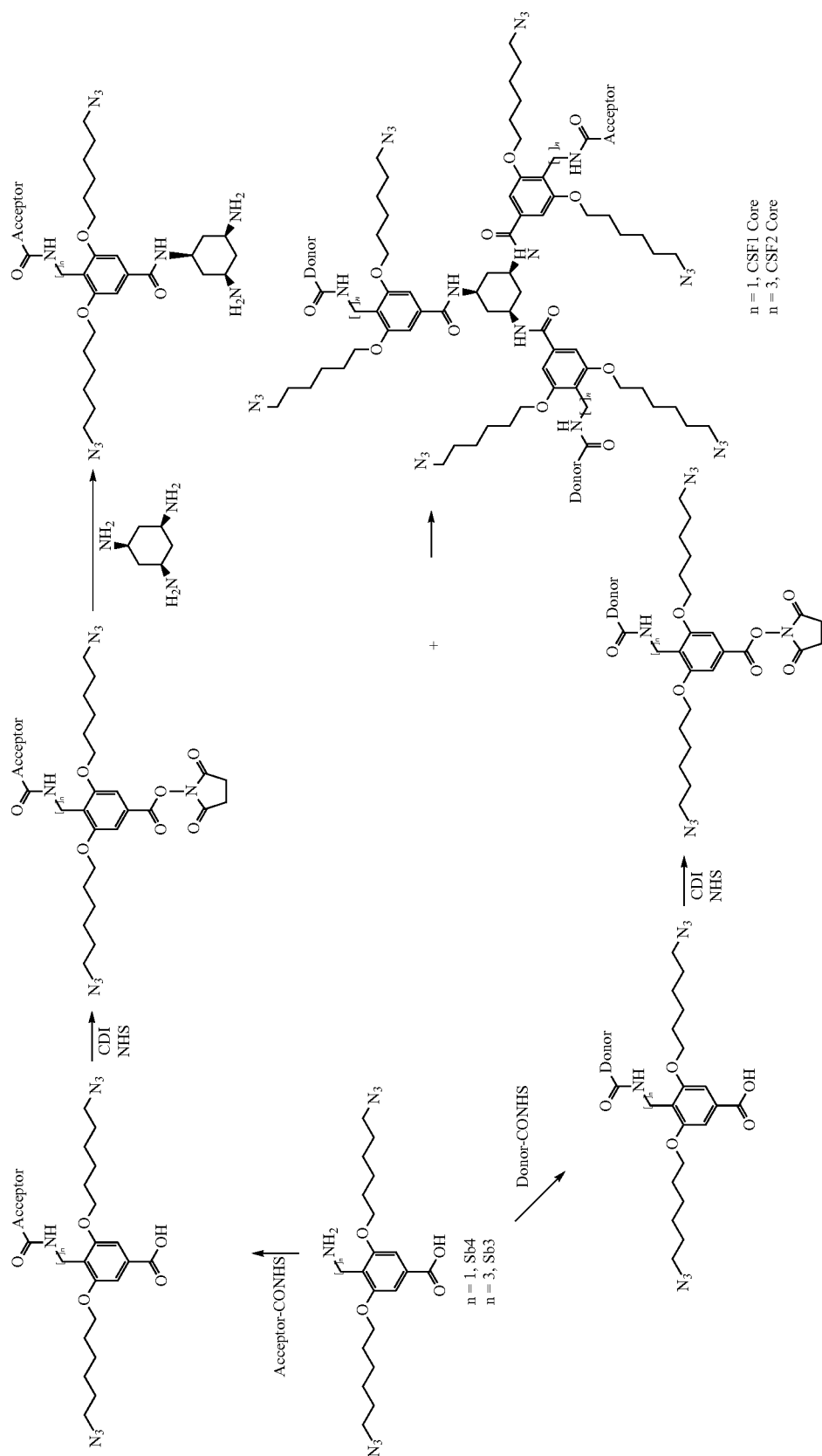
Scheme 10
