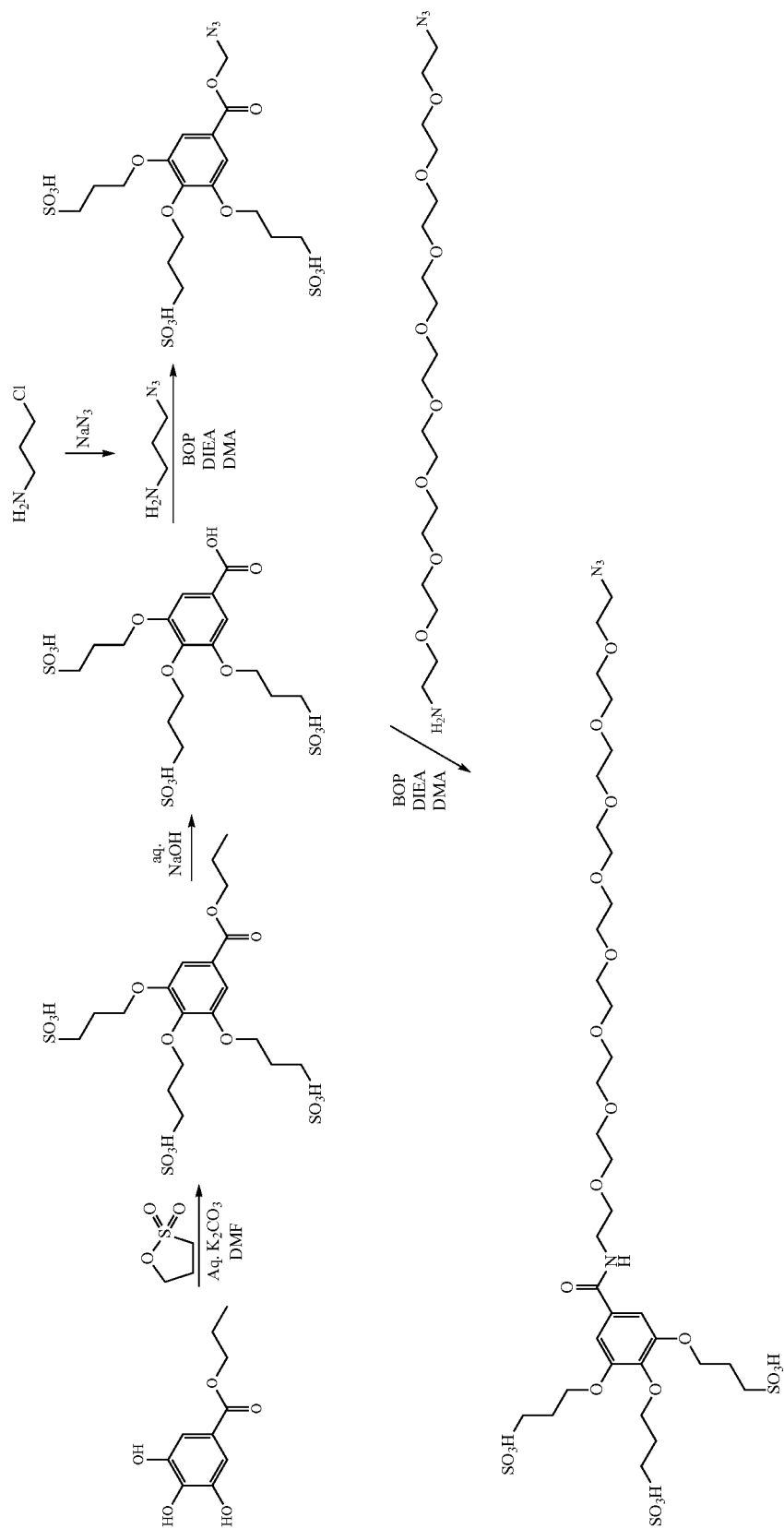
Scheme 15-2
