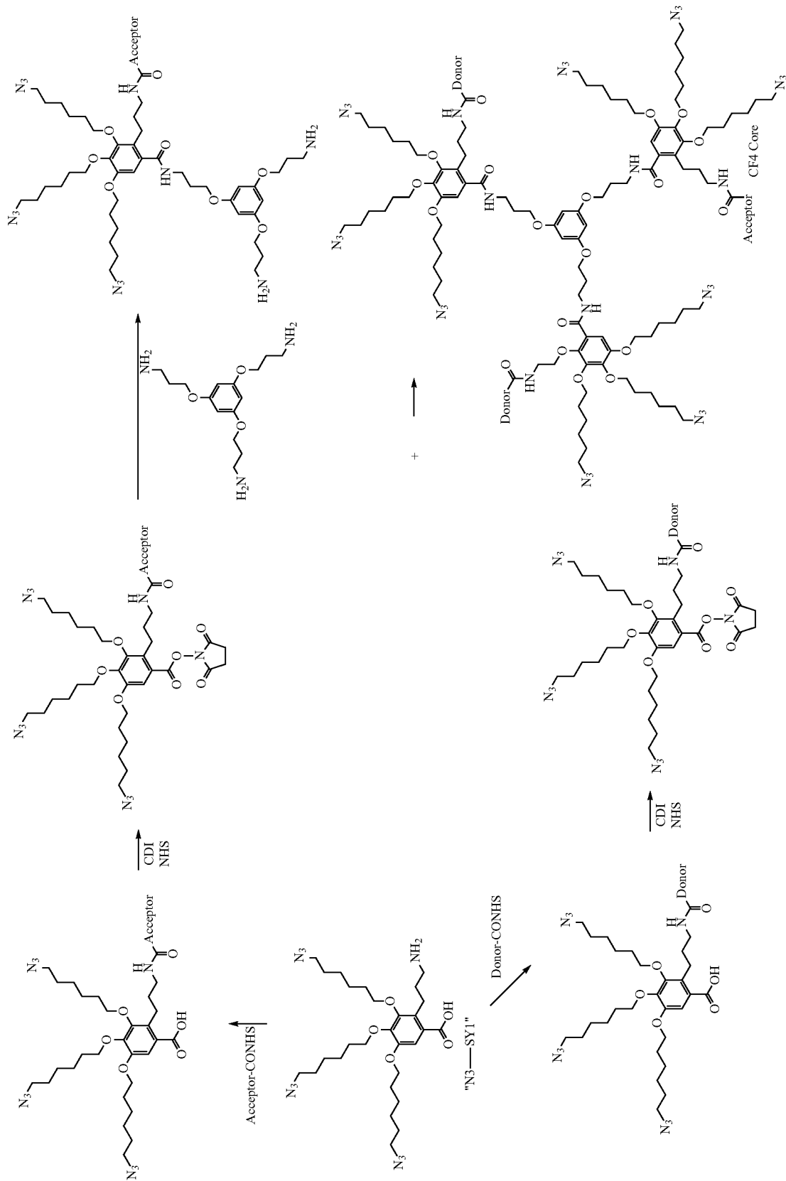
Scheme 11
