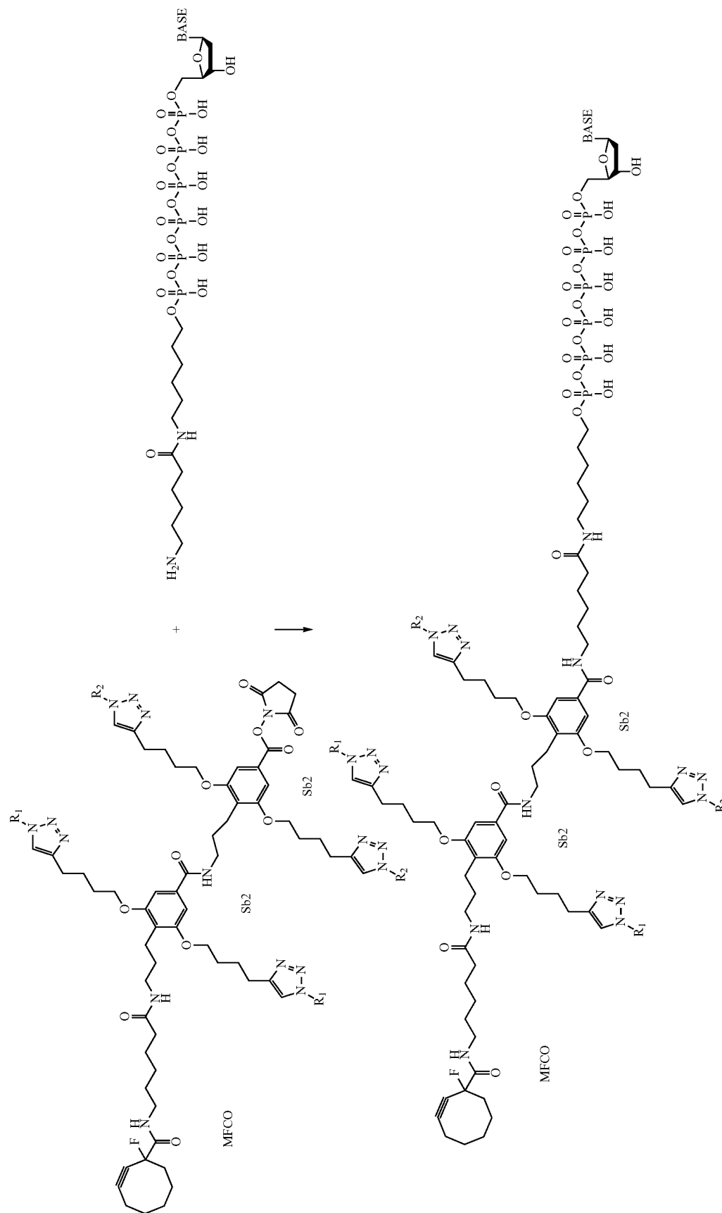
Scheme 14-2
