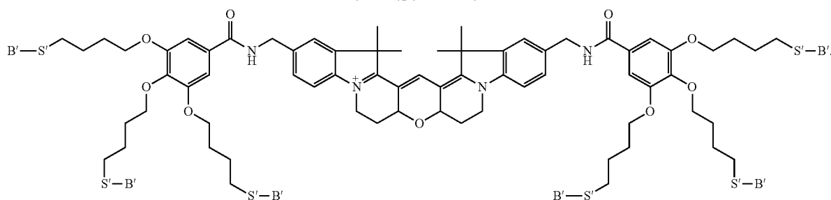
D012-(Gal) 2 (Hexavalent)
