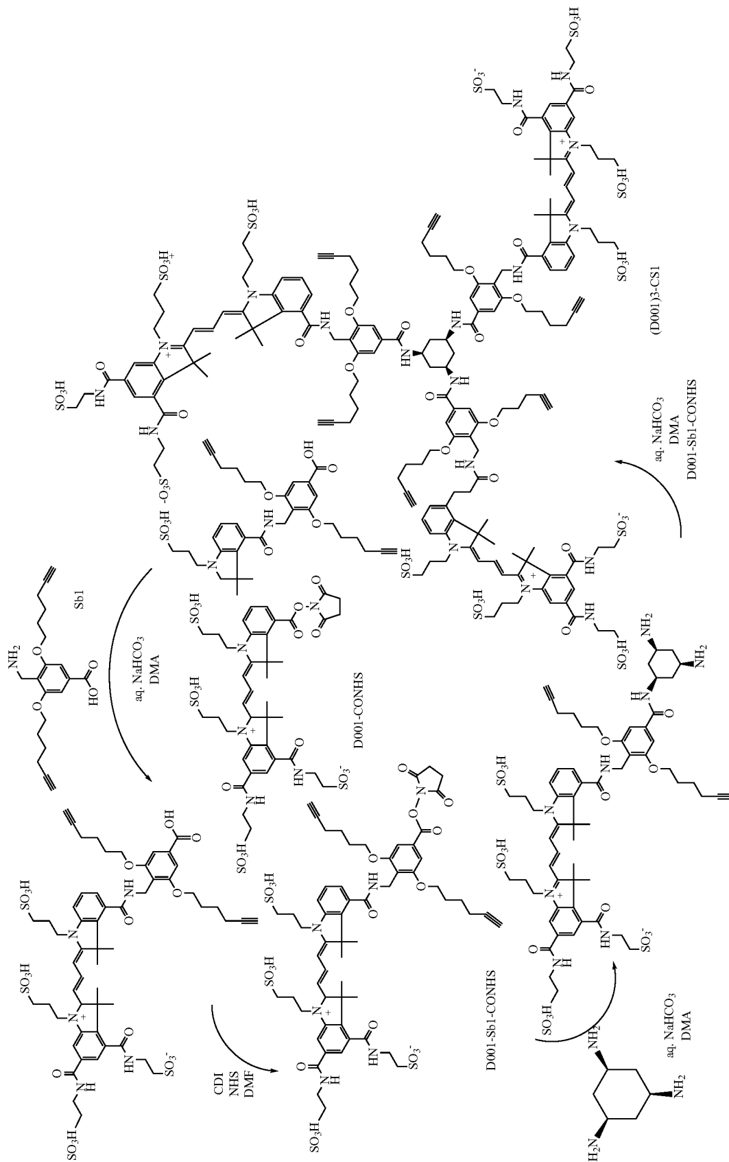
Scheme 2
