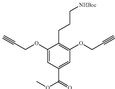
Methyl 4-(3-{{tert-butoxy}carbonyl}amino}propyl)-3,5-bis(prop-2-yn-1-yloxy)benzoate (4-9)
