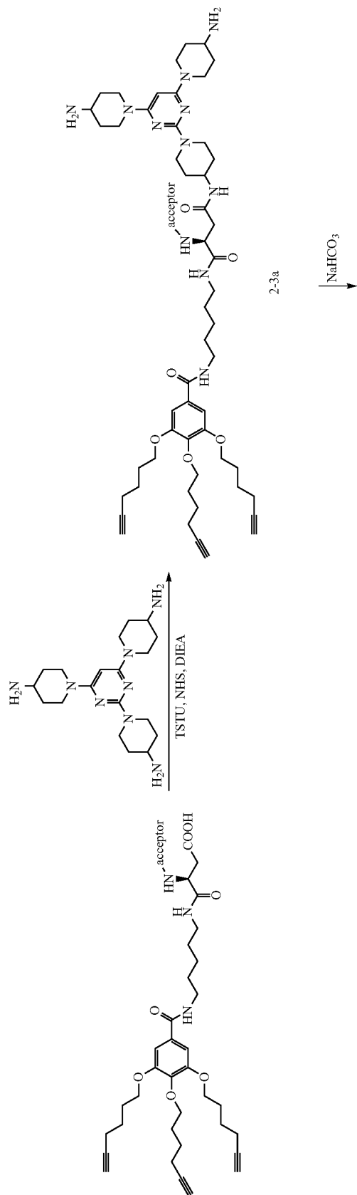
Scheme 18
