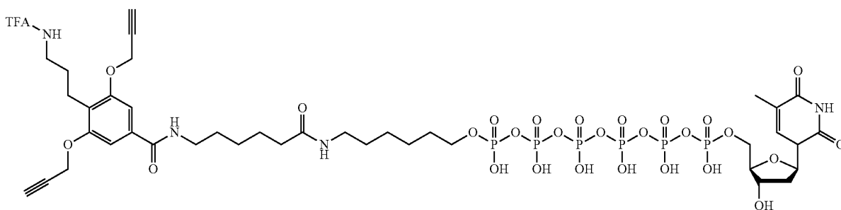
TFA-Sh-14C-dT6P (5-3)
