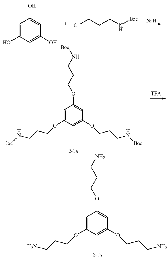
Scheme 16
