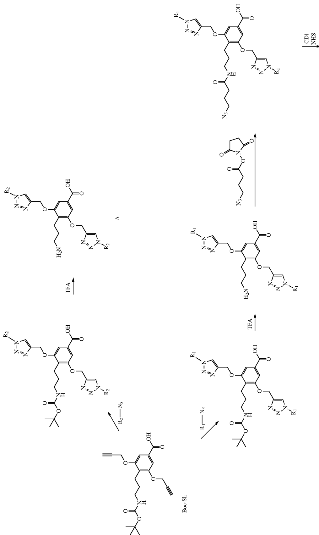
Scheme 7-4
