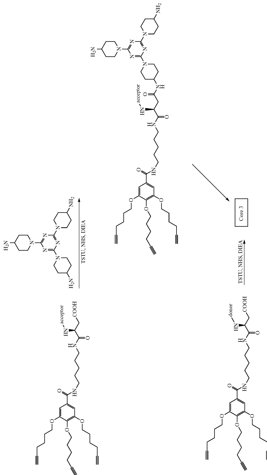
Scheme 6-2
