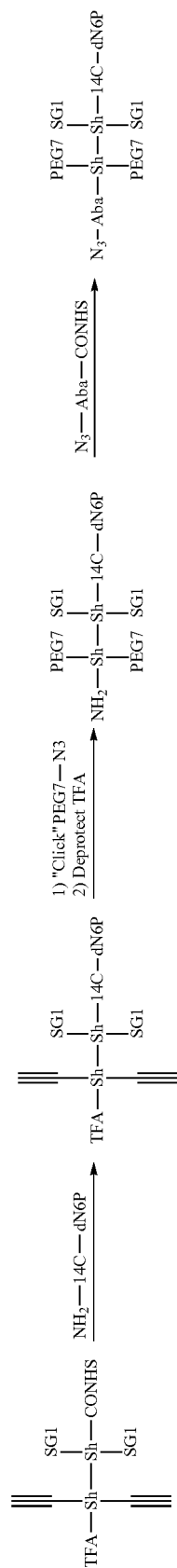
Scheme 7-2
