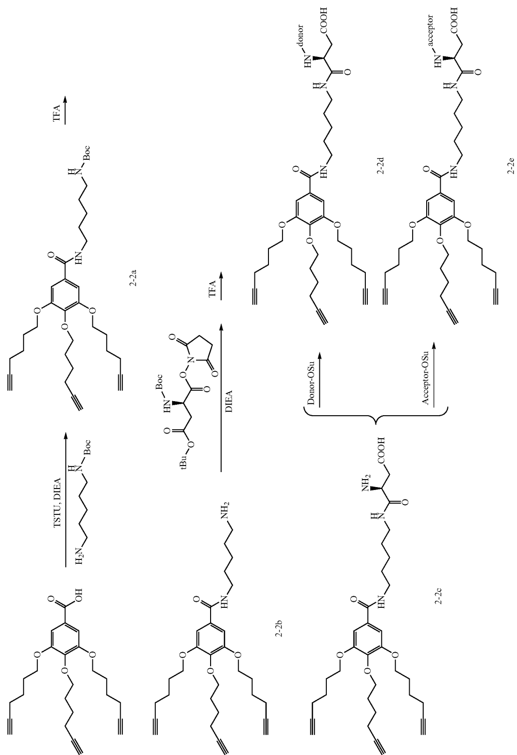
Scheme 17
