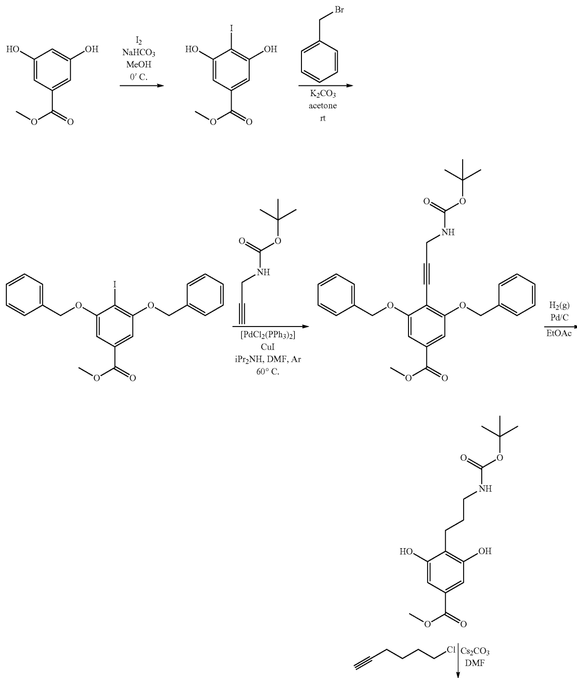
Scheme 15-1
