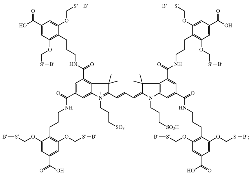
D010(Sh) 4 (Octavalent)
