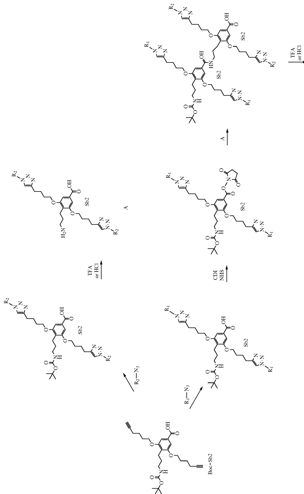
Scheme 14-1
