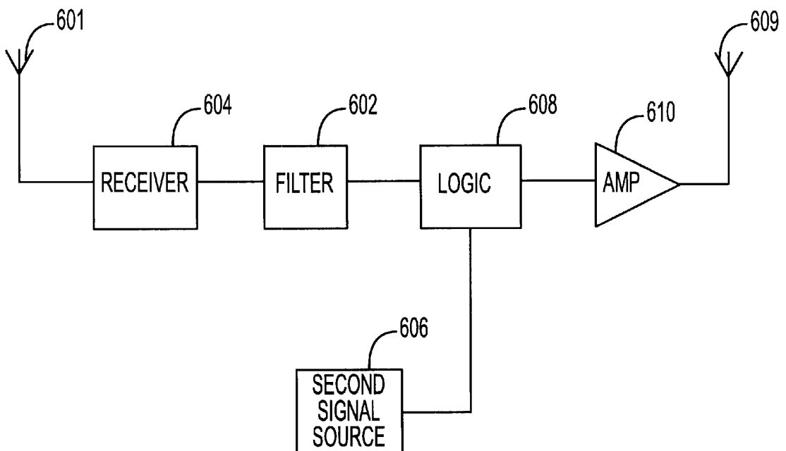
FIG. 6 (PRIOR ART)
