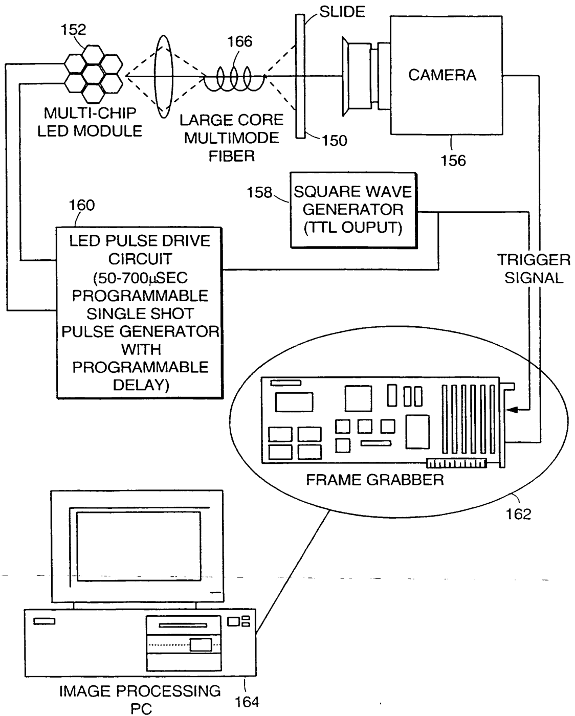
LED FIBER ILLUMINATION SYSTEM
