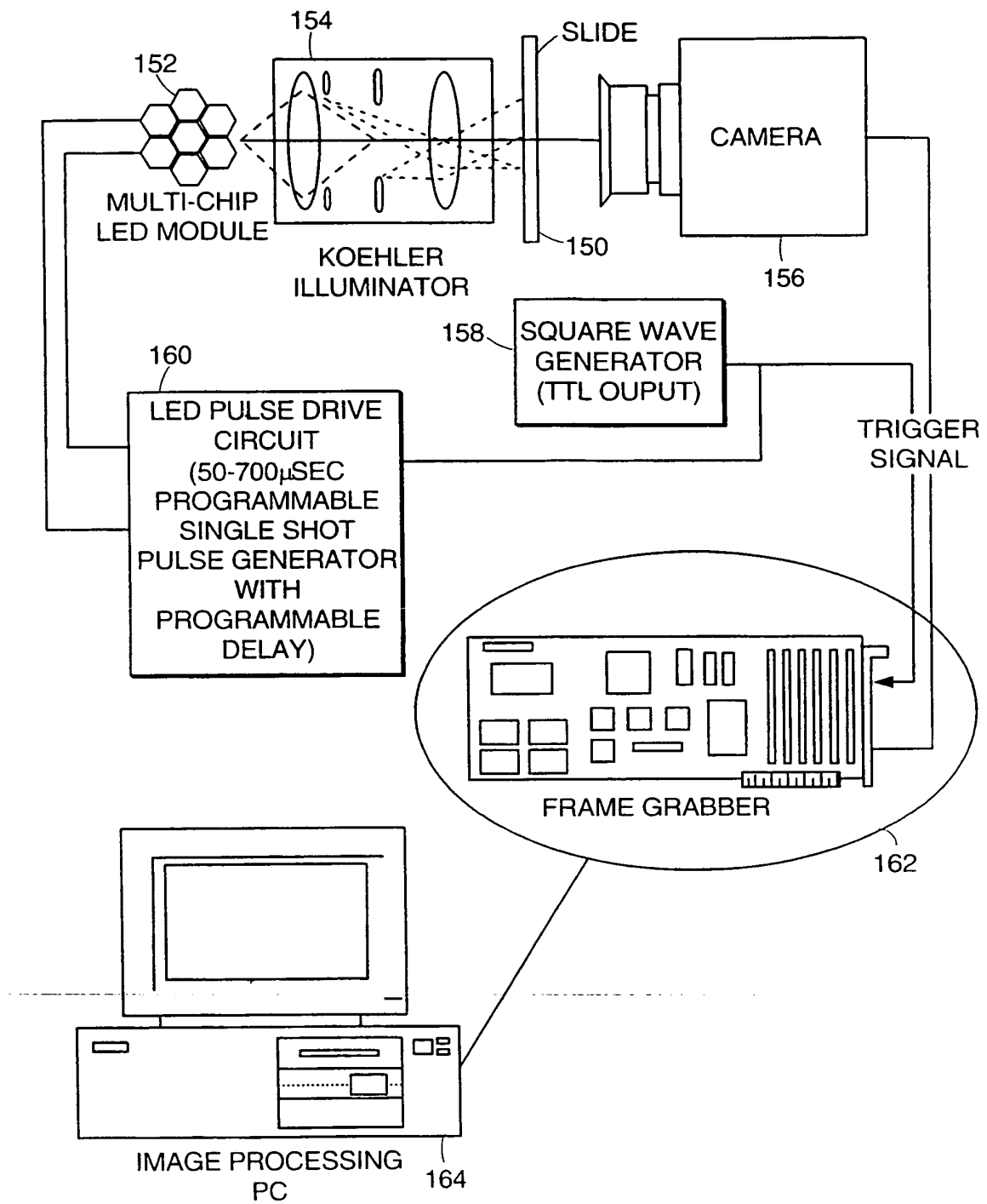
LED KOEHLER ILLUMINATION SYSTEM
