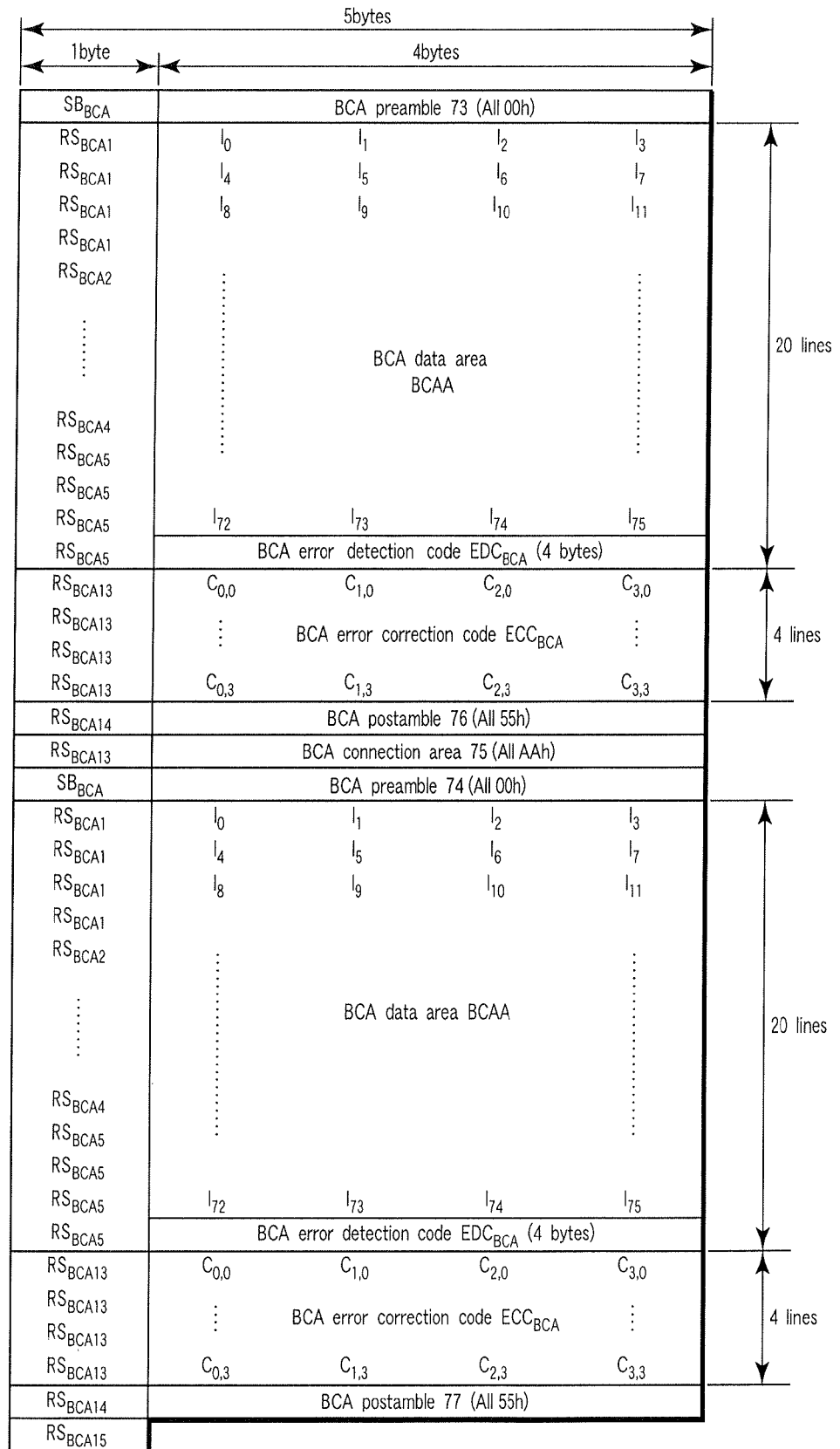
Illustrative view of BCA data structure
