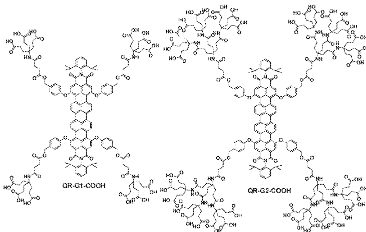
Structures of QR-G1-COOH and QR-G2-COOH .
