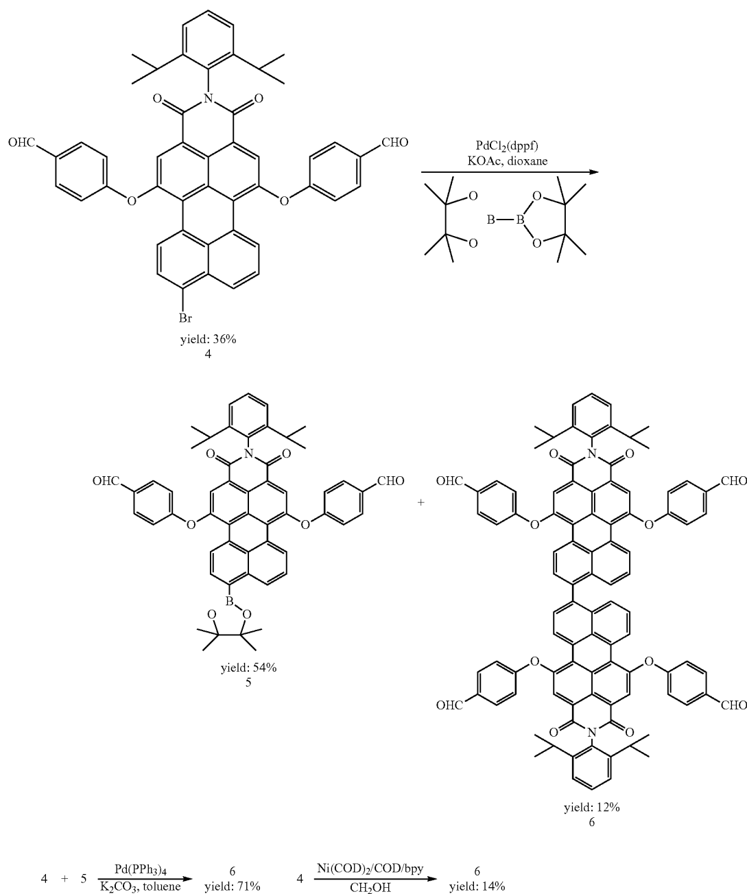
Scheme 1 Synthesis of QR-G1-COOH and QR-G2-COOH.
