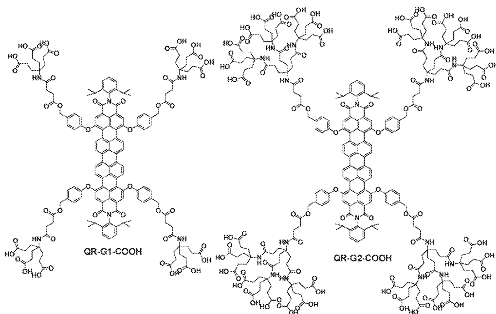
Fig. 1 Structures of QR-G1-COOH and QR-G2-COOH.
