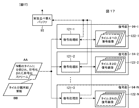
FIG. 17: 94 Decoder 95 Screen rearrangement buffer 121 Decoding processor 122-1 Tile #1 decoded image 122-2 Tile #2 decoded image 122-N Tile #N decoded image AA Encoding stream partitioned into N tiles and encoded BB Tile-partition-possibility information
