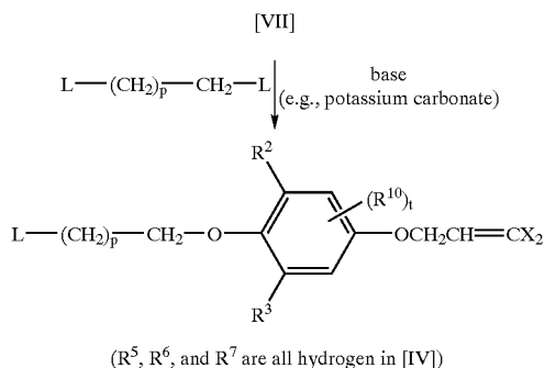
SCHEME 14
