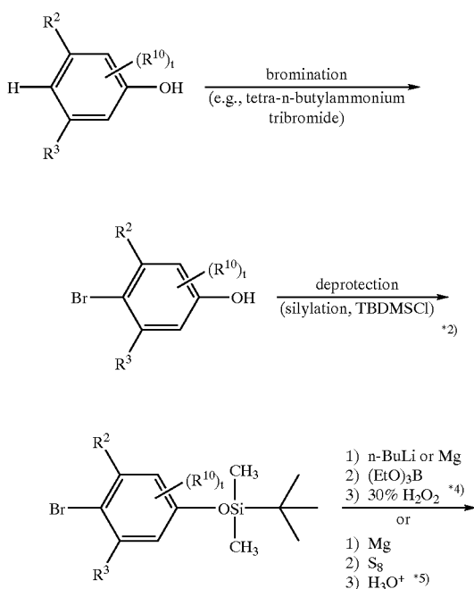
SCHEME 6
