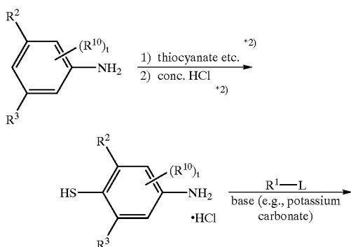
SCHEME 4
