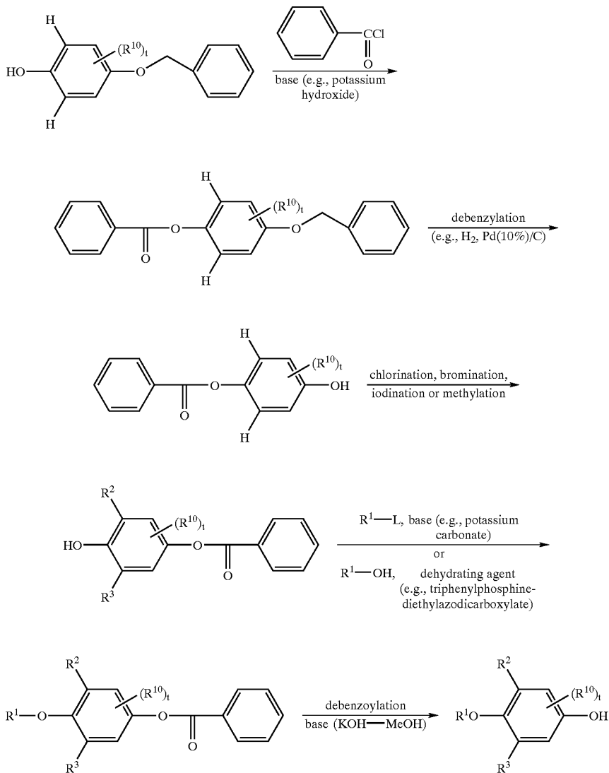
SCHEME 3
