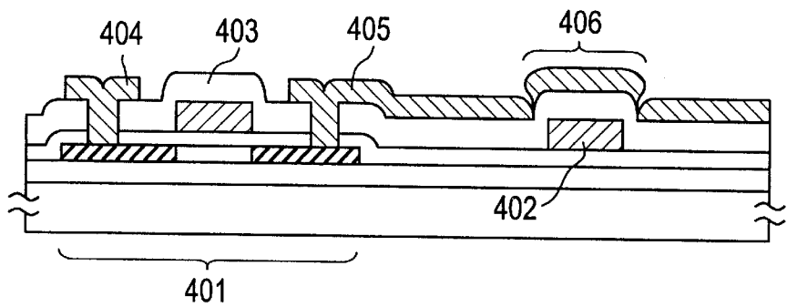
FIG. 4 PRIOR ART
