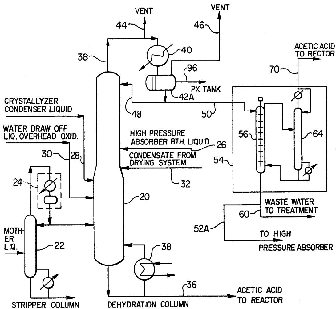
FIG. 3 (EXTRACTION SYSTEM)
