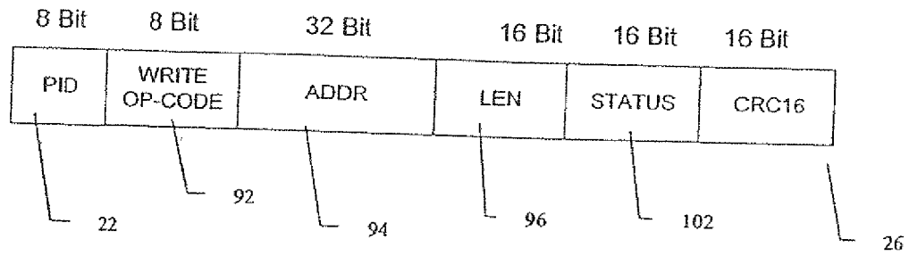
Fig 10 - Write Status Packet
