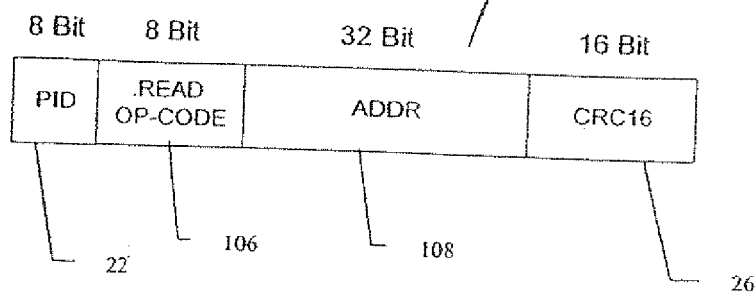
Fig 11 - Read Request Packet
