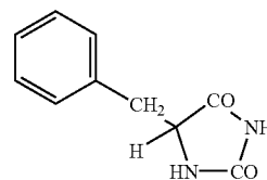
DL-5-SUBSTITUTED HYDANTOIN
