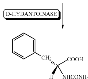
N-CARBAMYL-D-AMINO ACID
