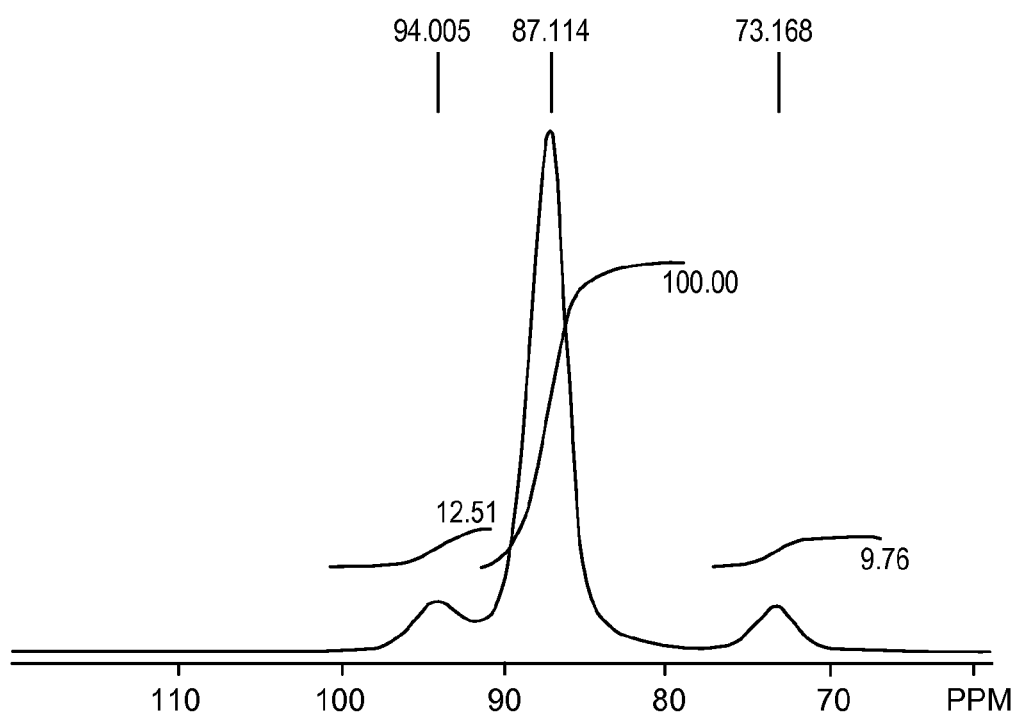
FIGURE 23C: LSPS ^{31}\text{P} NMR
