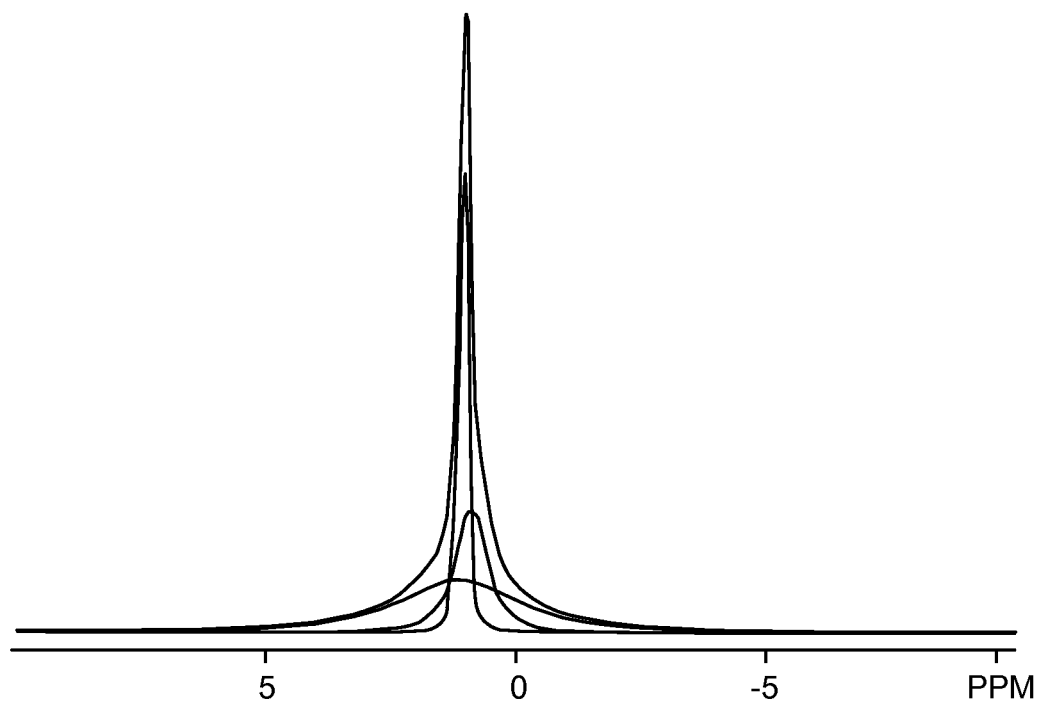
FIGURE 22C: LSPS {}^7\text{Li} NMR
