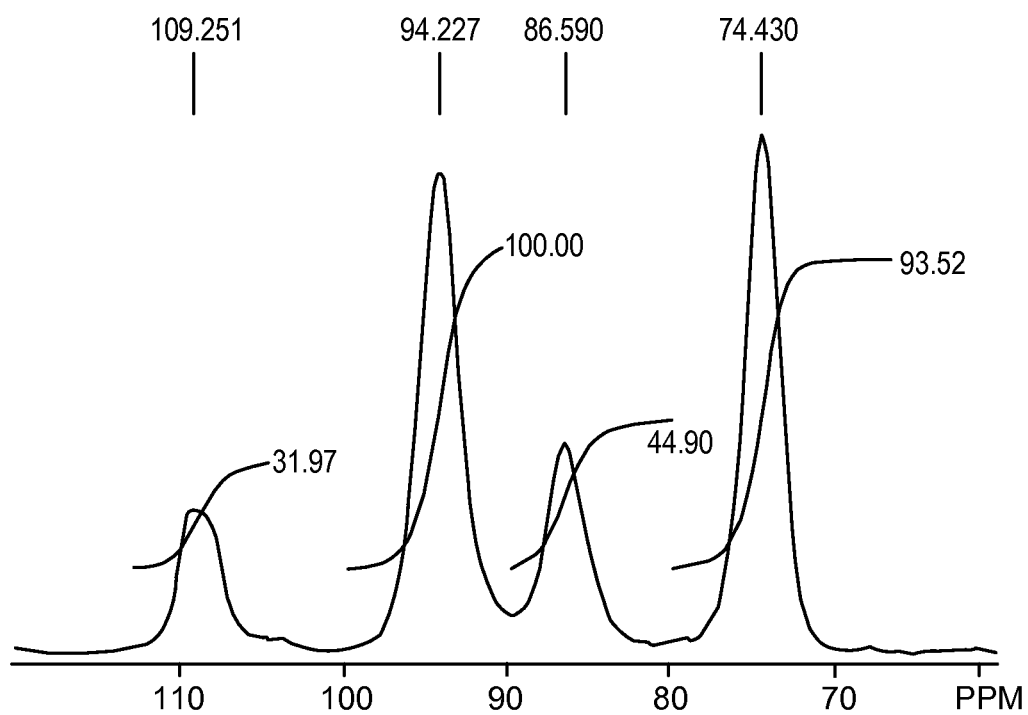
FIGURE 23D: LGPS ^{31}\text{P} NMR
