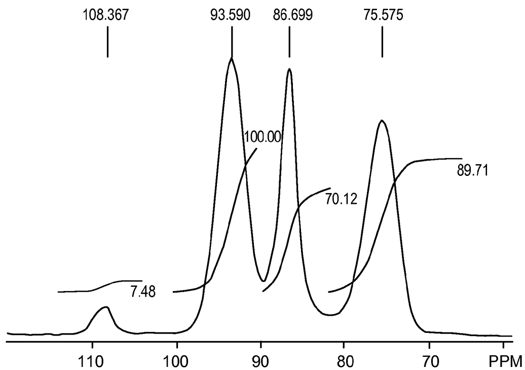
FIGURE 23B: LSTPS ^{31}\text{P} NMR
