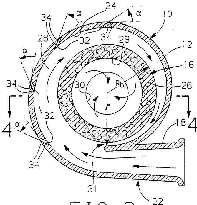
IDEAL UNIFORM MASS FLOW-DISTRIBUTION PRIOR ART FIG. 2
