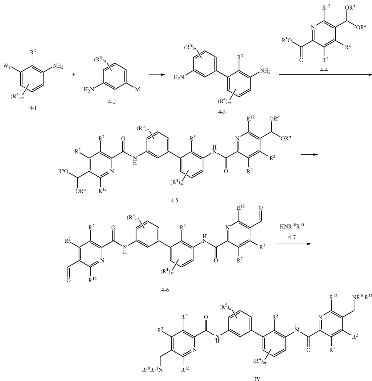
Scheme 4
