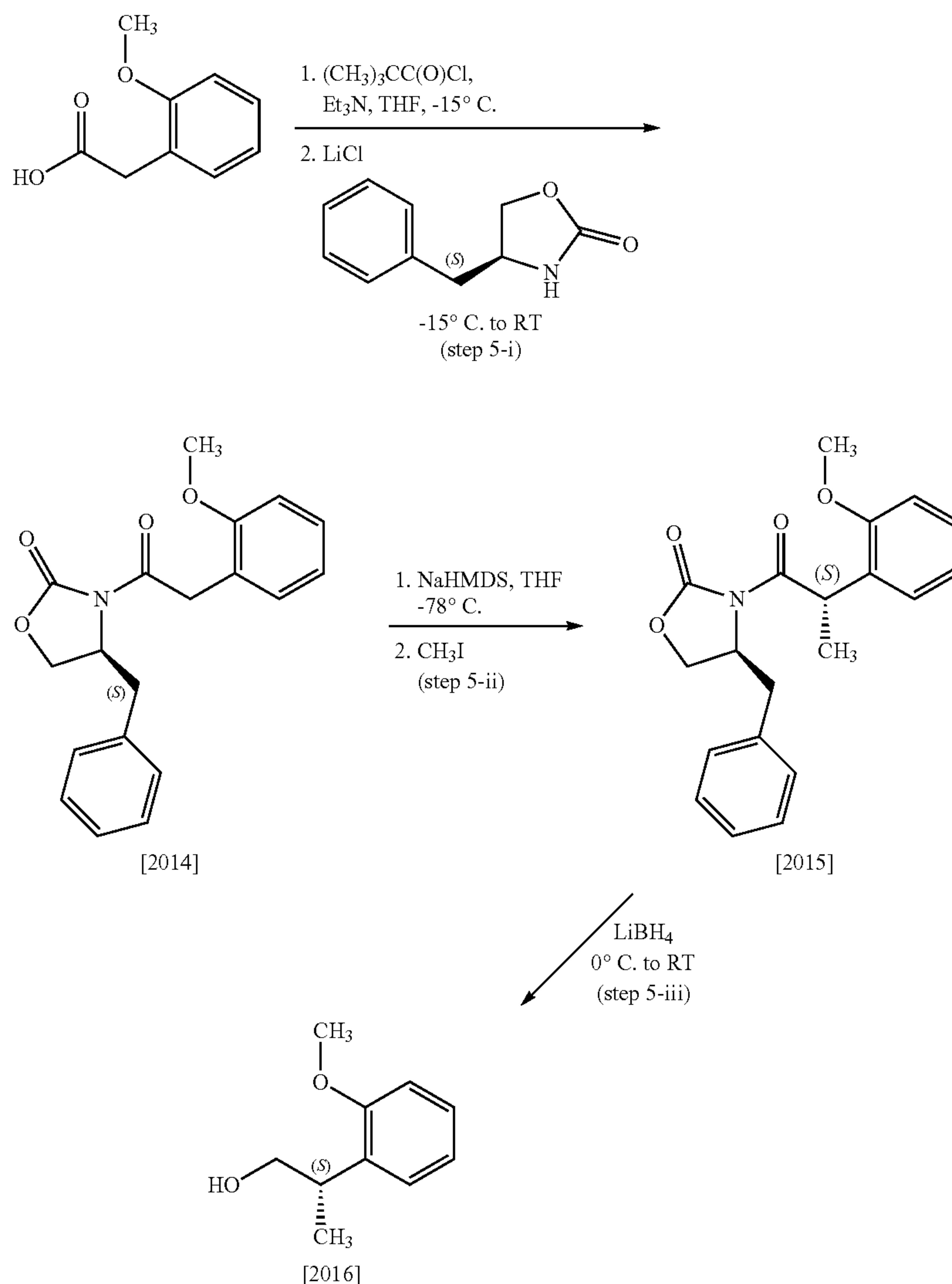
Scheme 5
