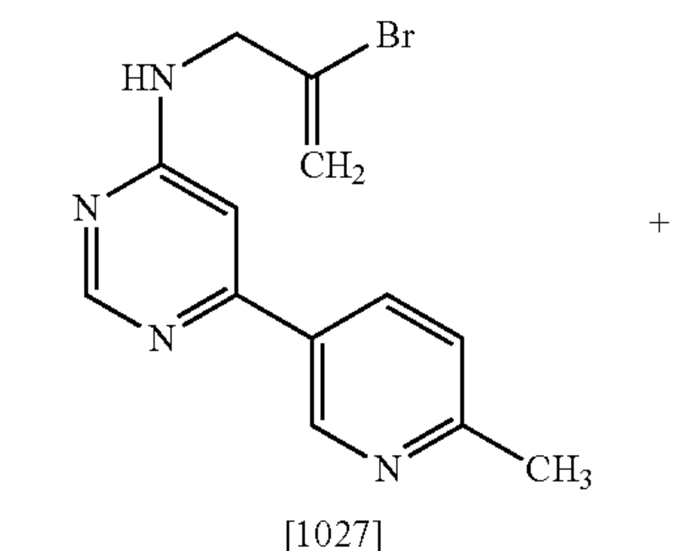
Scheme 8
