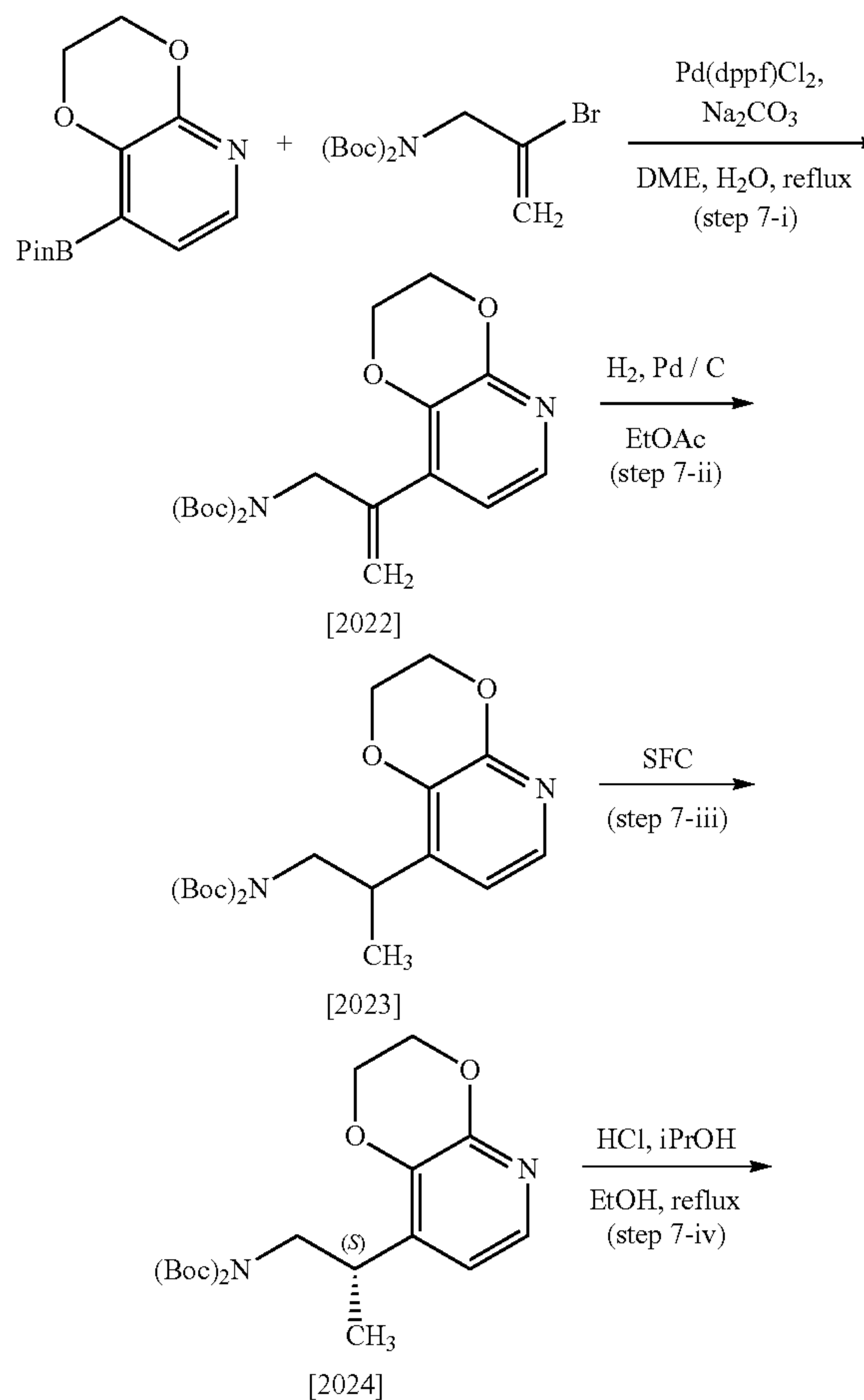
Scheme 7
