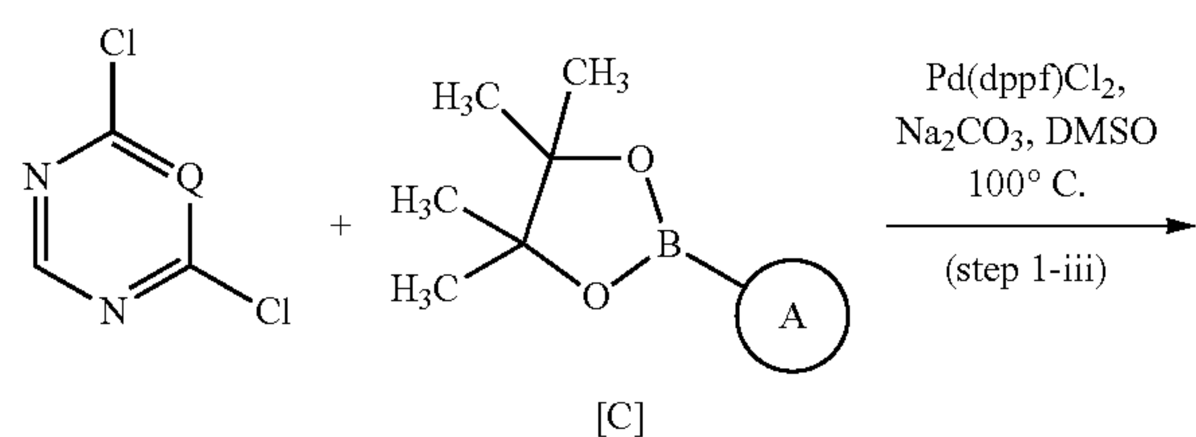
Scheme 1 - Method B
