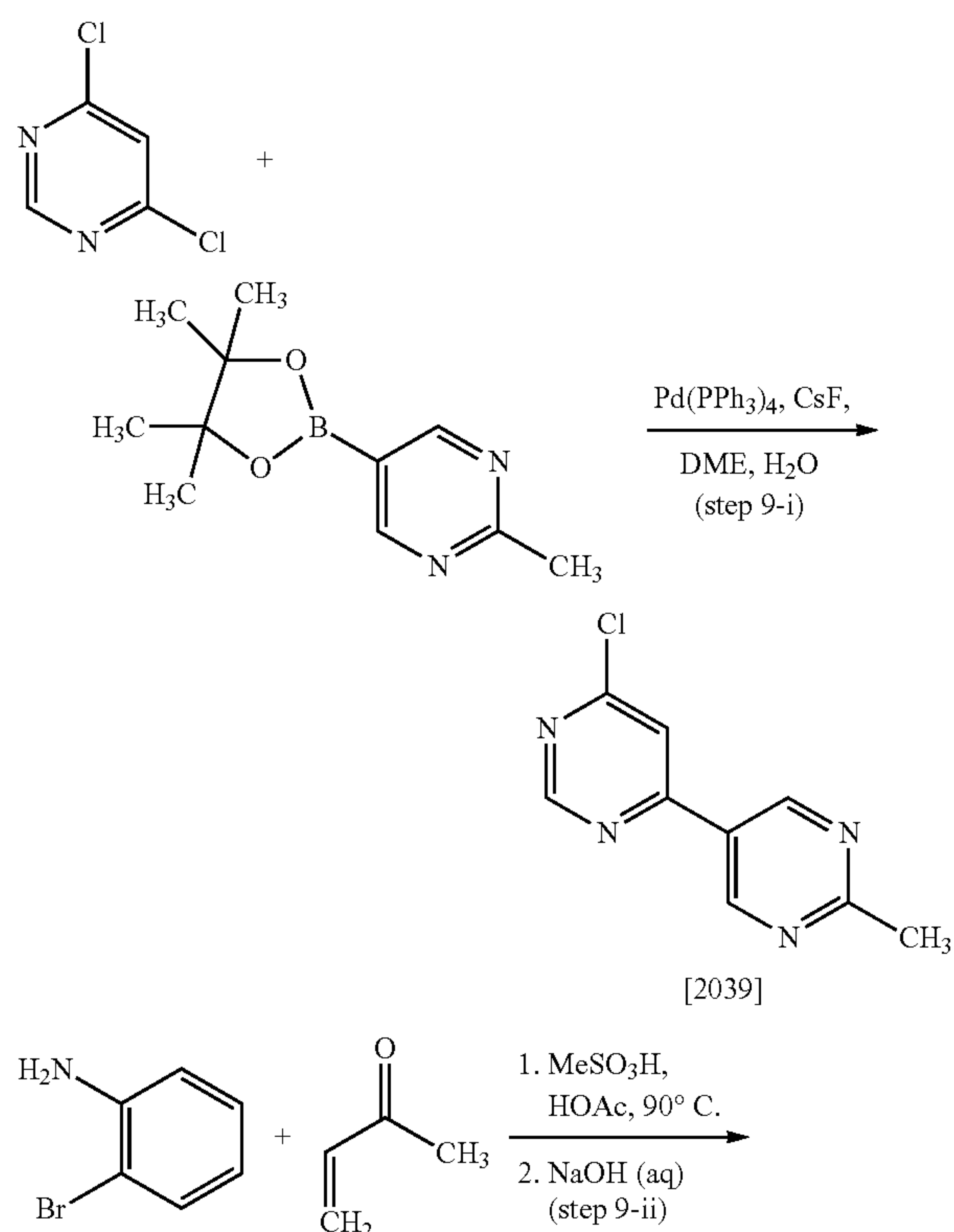
Scheme 9
