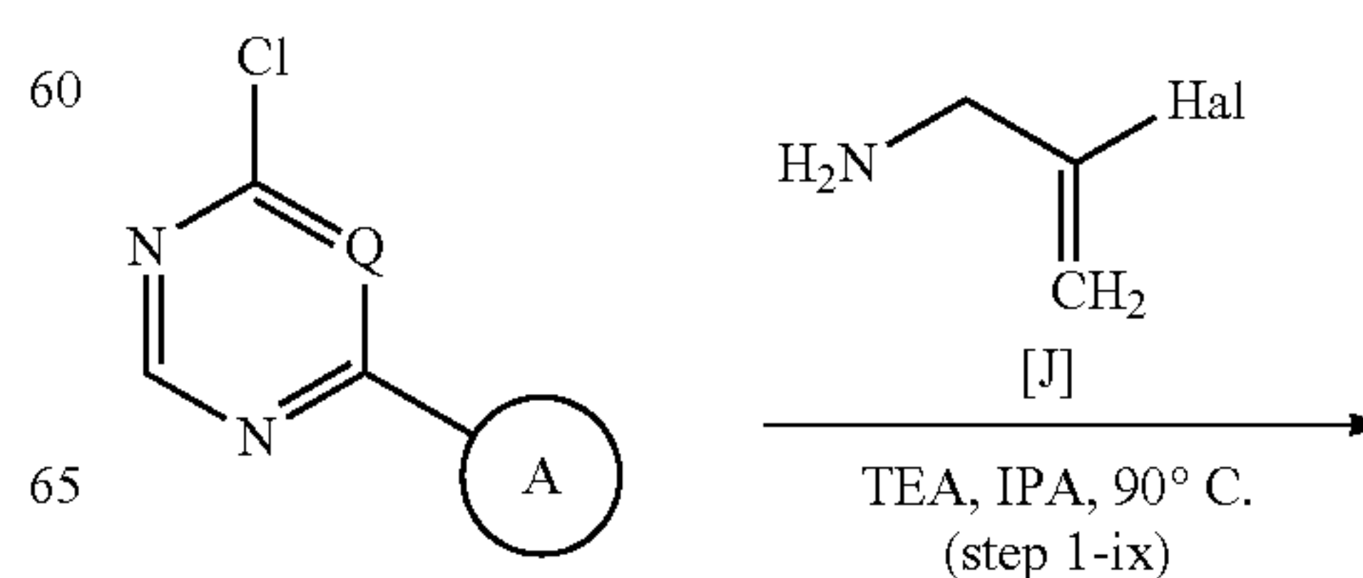
Scheme 1 - Method D
