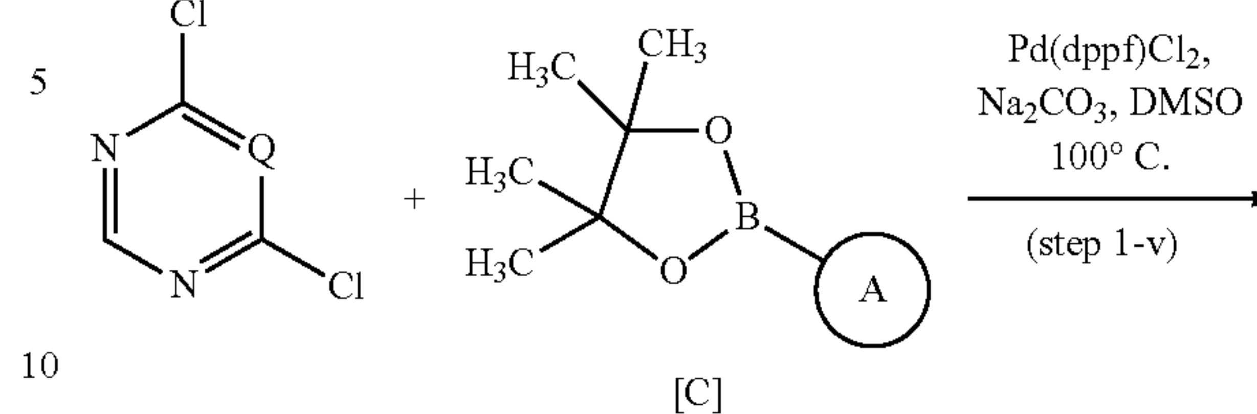
Scheme 1 - Method C
