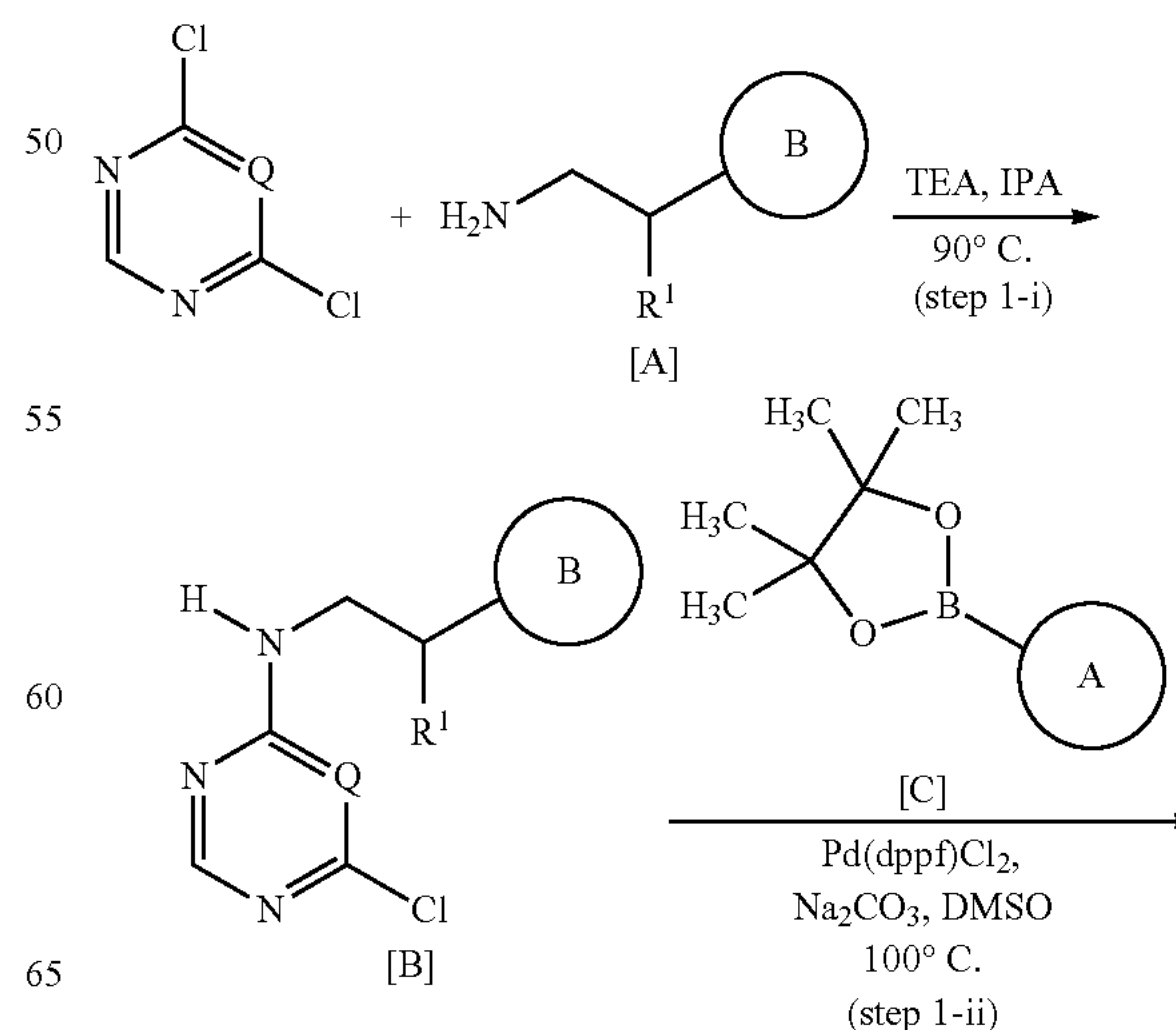
Scheme 1-Method A
