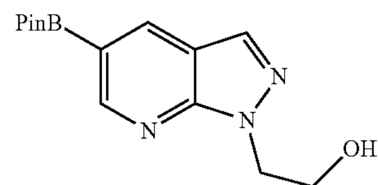
2-(5-(4,4,5,5-tetramethyl-1,3,2-dioxaborolan-2-yl)-1H-pyrazolo[3,4-b]pyridin-1-yl)ethanol
