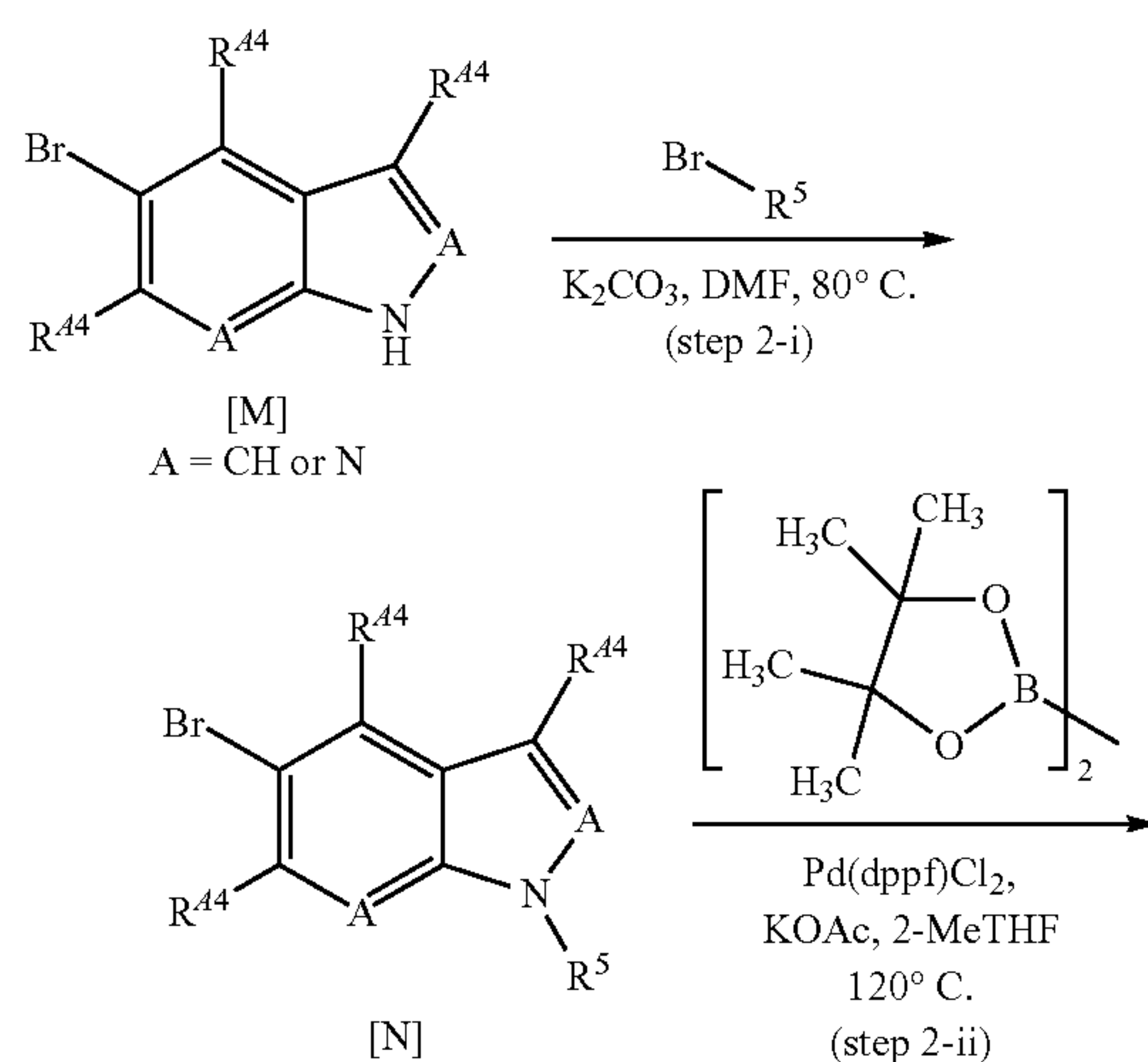
Scheme 2
