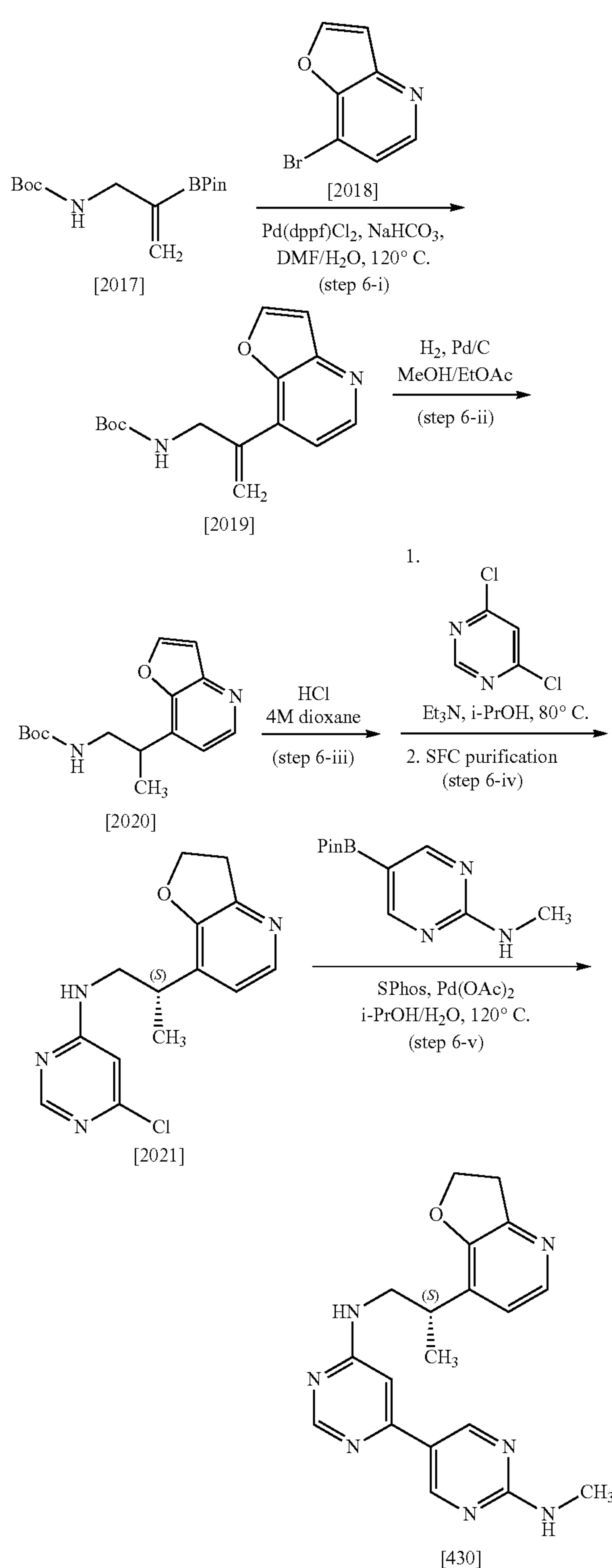
Scheme 6
