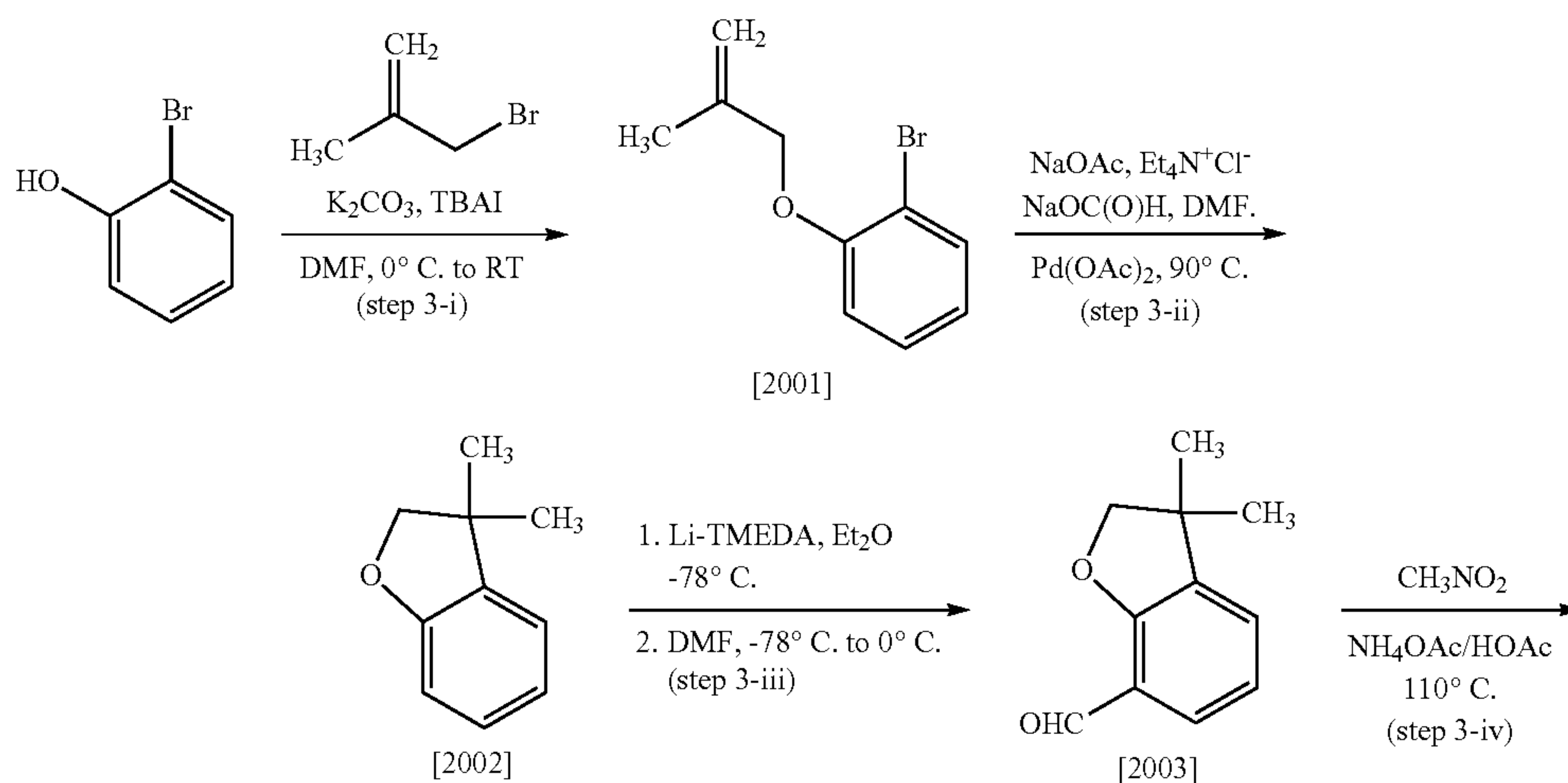
Scheme 3
