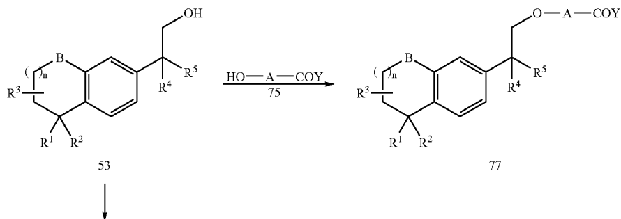
Scheme 6
