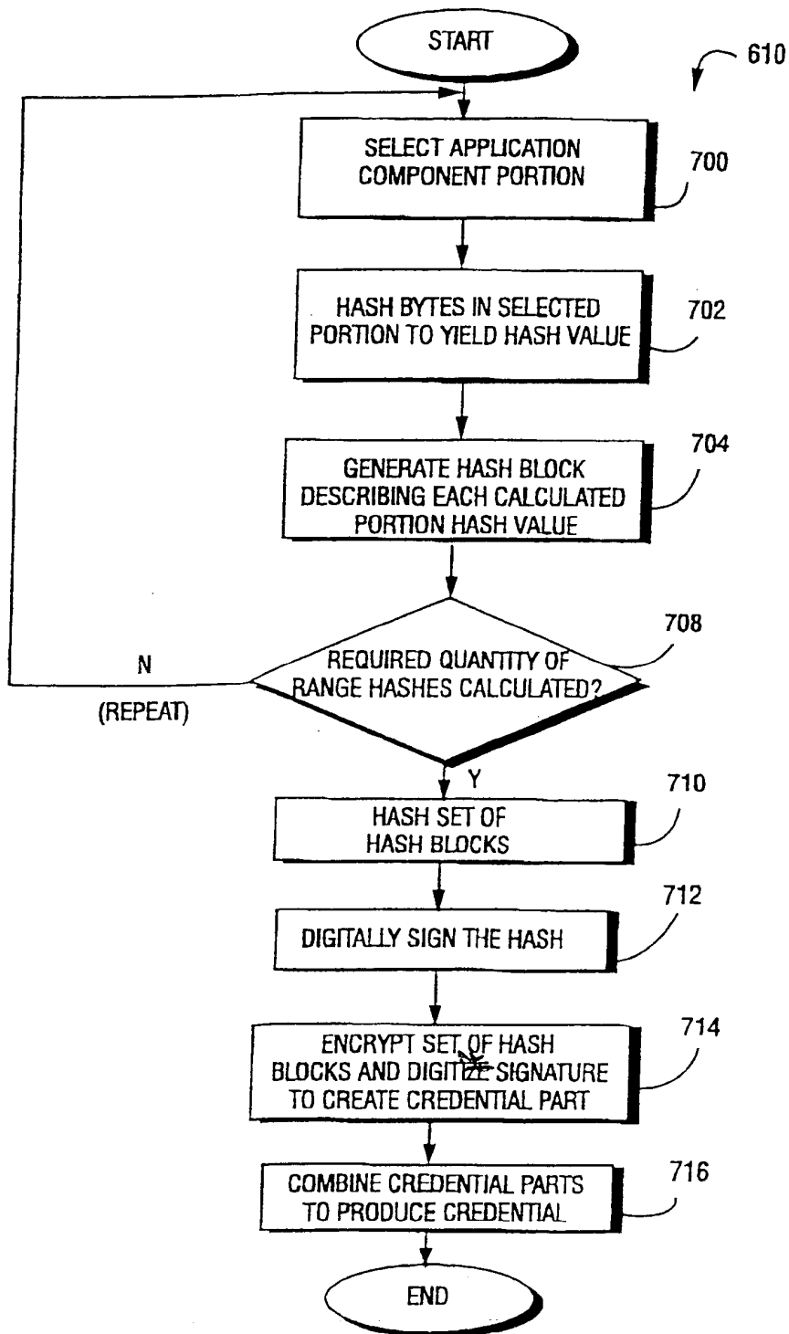
FIG. 17 EXAMPLE CREDENTIAL CREATION PROCESS
