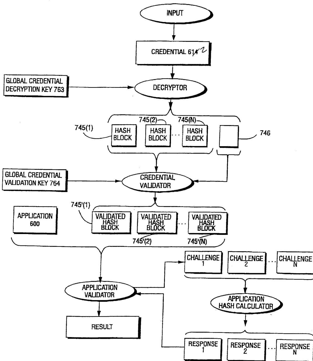
FIG. 22B EXAMPLE CREDENTIAL VALIDATION
