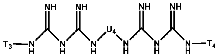
[Chemical Formula 10]
