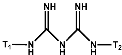
[Chemical Formula 10]
