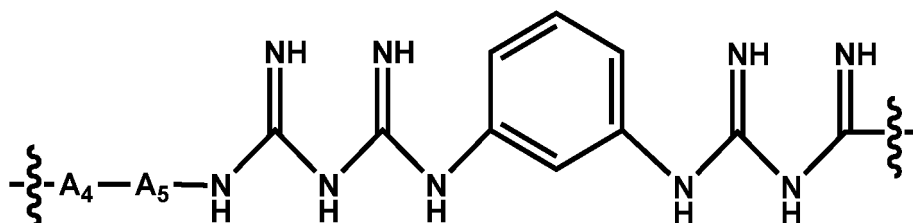
[Chemical Formula 2-2]
