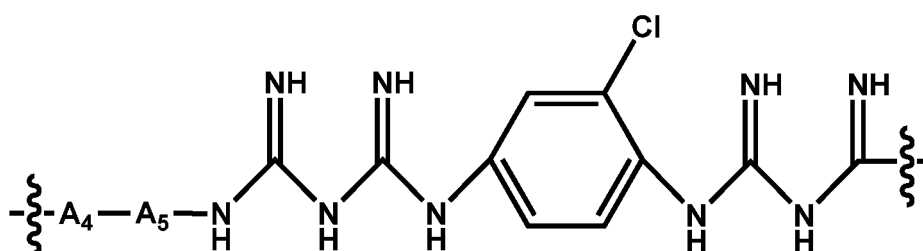
[Chemical Formula 2-4]
