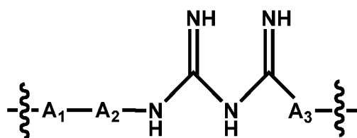
[Chemical Formula 1]
