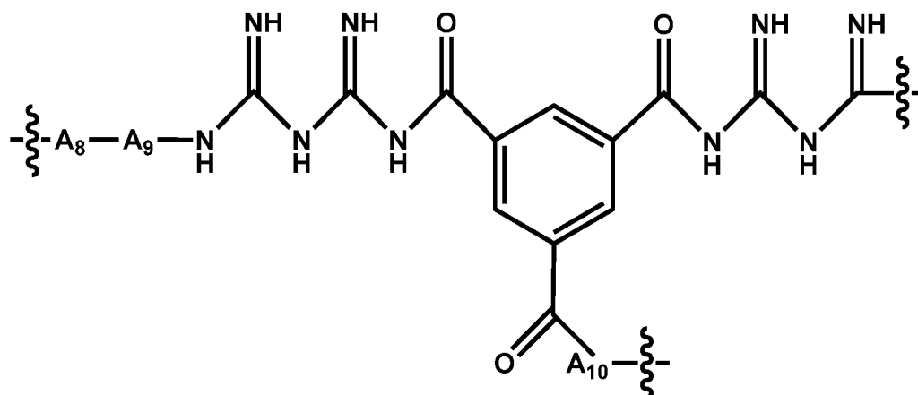
[Chemical Formula 4-1]
