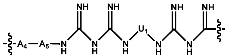
[Chemical Formula 2]
