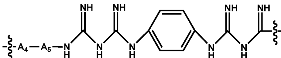
[Chemical Formula 2-2]
