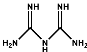
[Chemical Formula 9-1]
