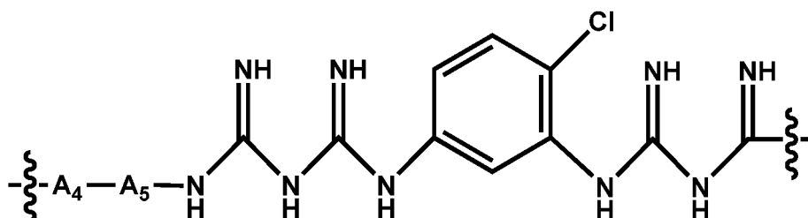
[Chemical Formula 2-3]
