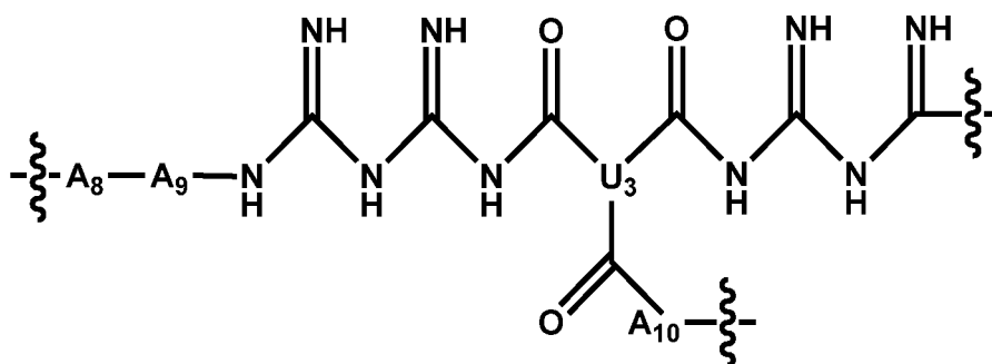
[Chemical Formula 4]
