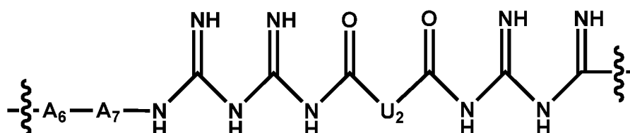
[Chemical Formula 3]
