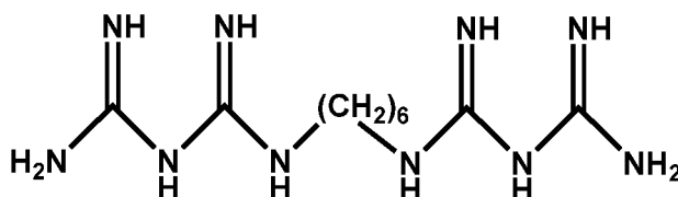
[Compound B]
