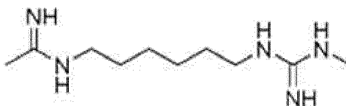
PHB Monomer
