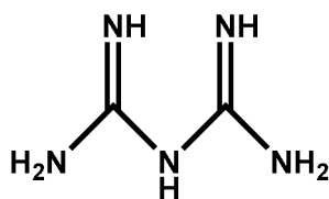
[Compound B]
