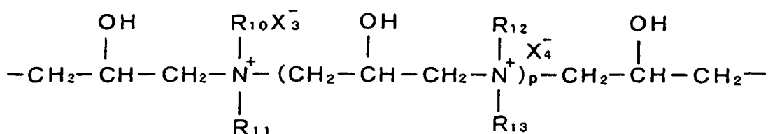
General formula (4)
