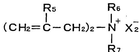
General formula (2)
