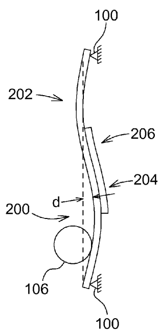
FIG. 9 Prior Art
