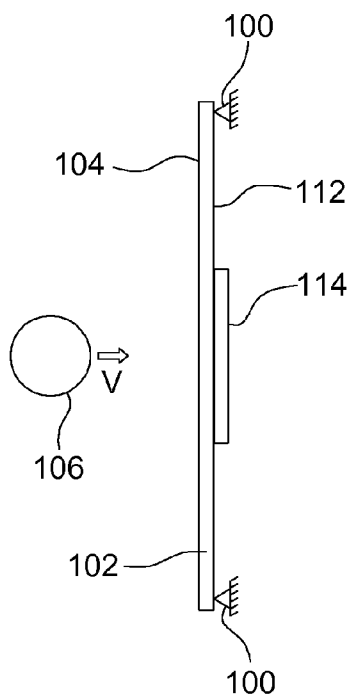
FIG. 3 Prior Art
