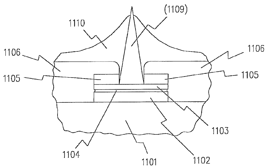
FIGURE 11b ELECTRODES
