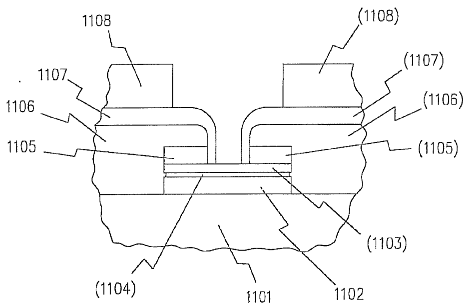
FIGURE 11a ELECTRODES
