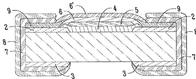
Fig. 3 PRIOR ART
