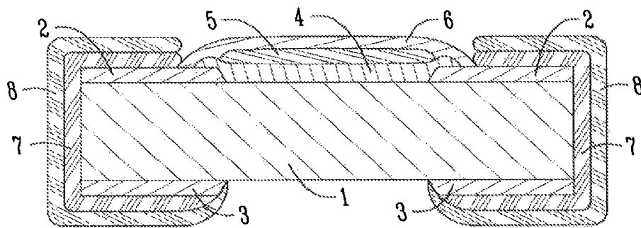
Fig. 2 PRIOR ART
